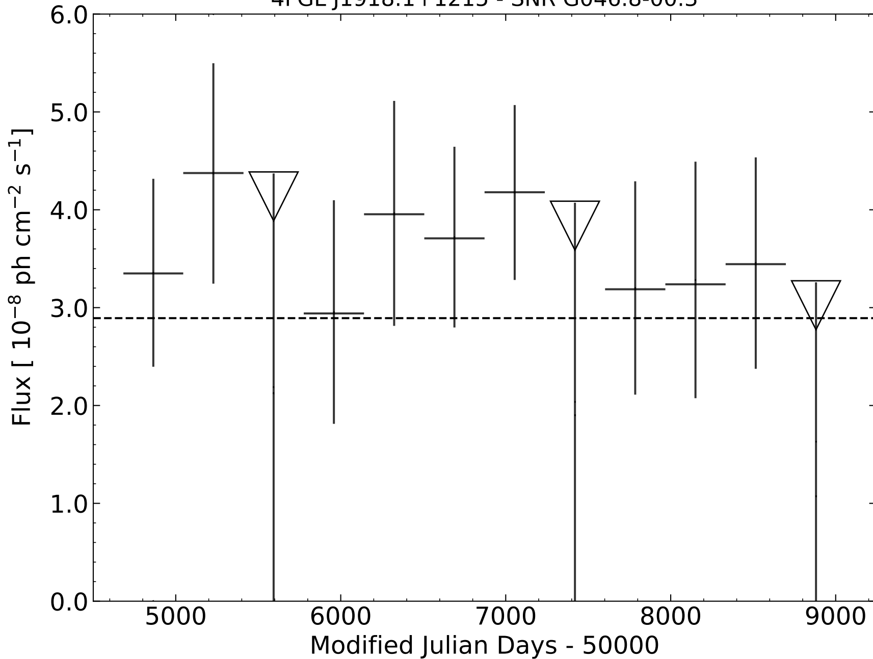
4FGL J1918.1+1215 - SNR G046.8-00.3
