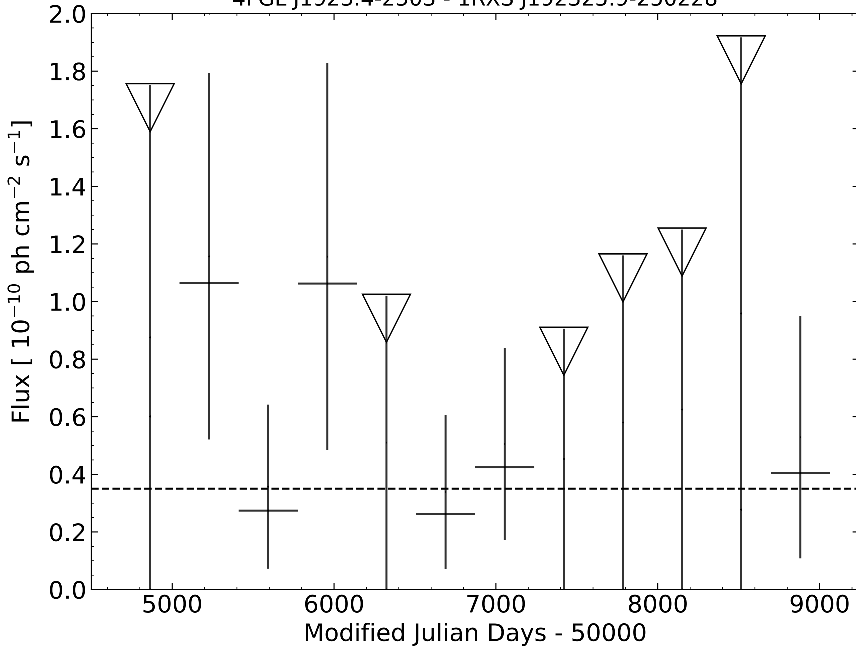
4FGL J1923.4-2503 - 1RXS J192325.9-250228
