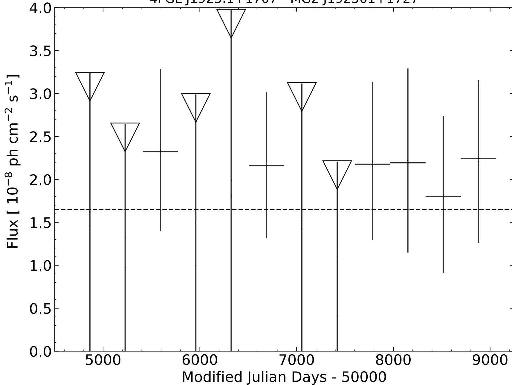
4FGL J1925.1+1707 - MG2 J192501+1727
