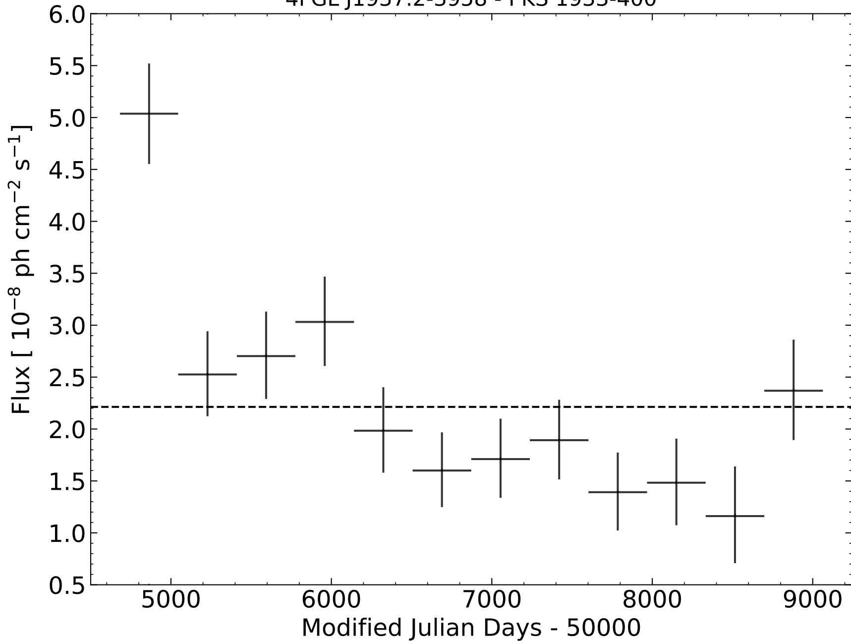
4FGL J1937.2-3958 - PKS 1933-400
