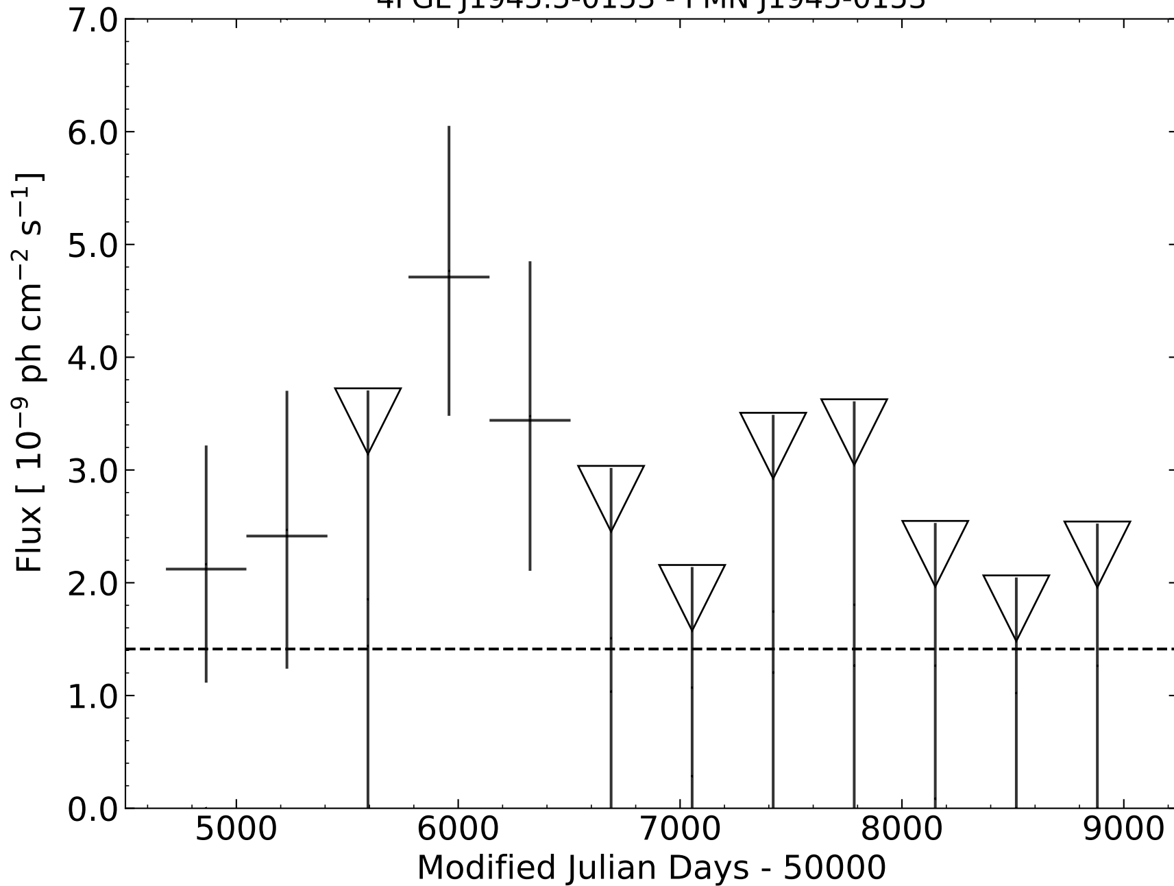
4FGL J1945.5-0153 - PMN J1945-0153
