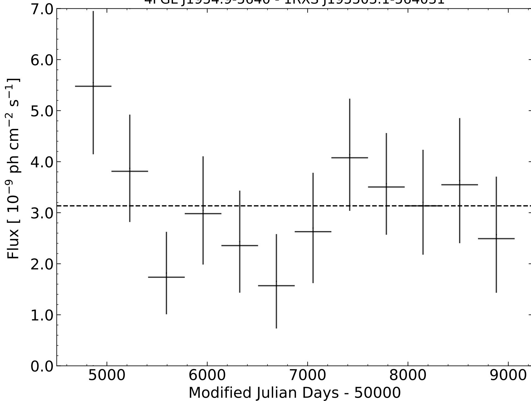
4FGL J1954.9-5640 - 1RXS J195503.1-564031
