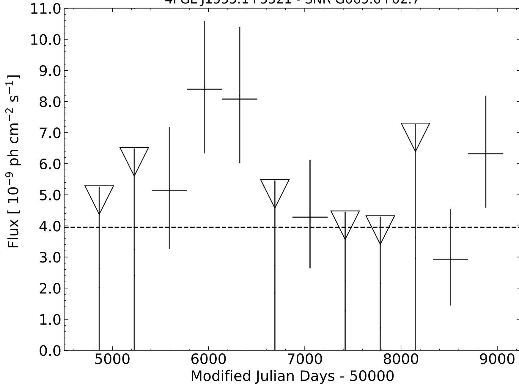
4FGL J1955.1+3321 - SNR G069.0+02.7
