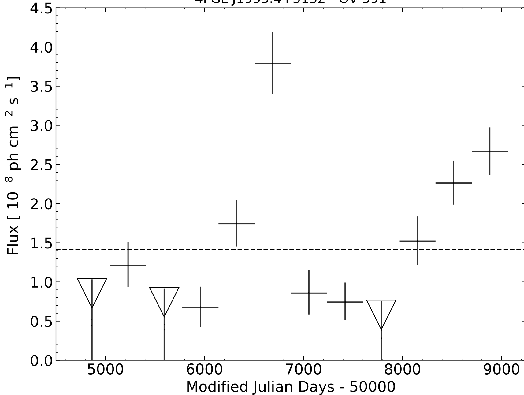
4FGL J1955.4+5132 - OV 591
