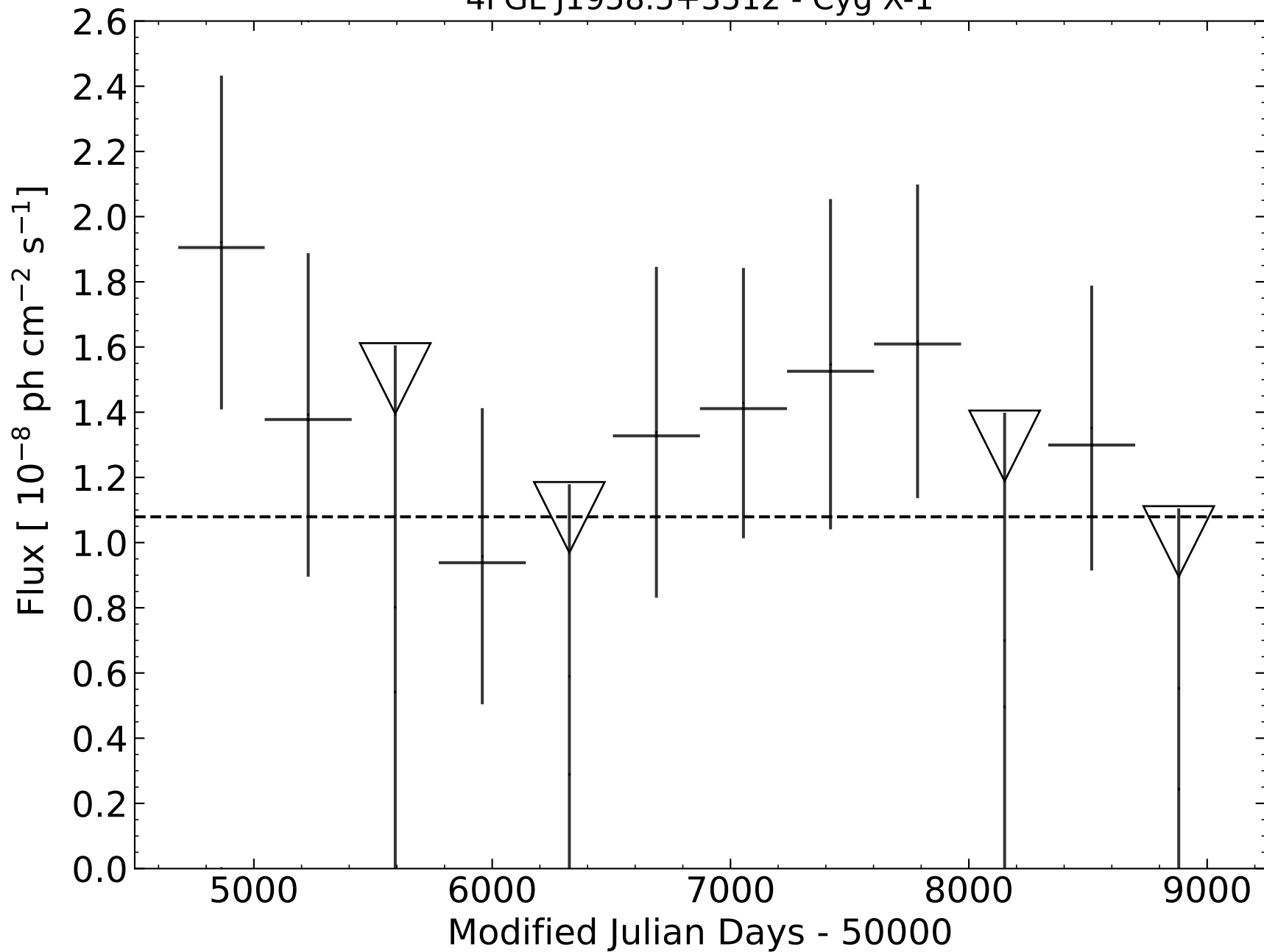
4FGL J1958.5+3512 - Cyg X-1
