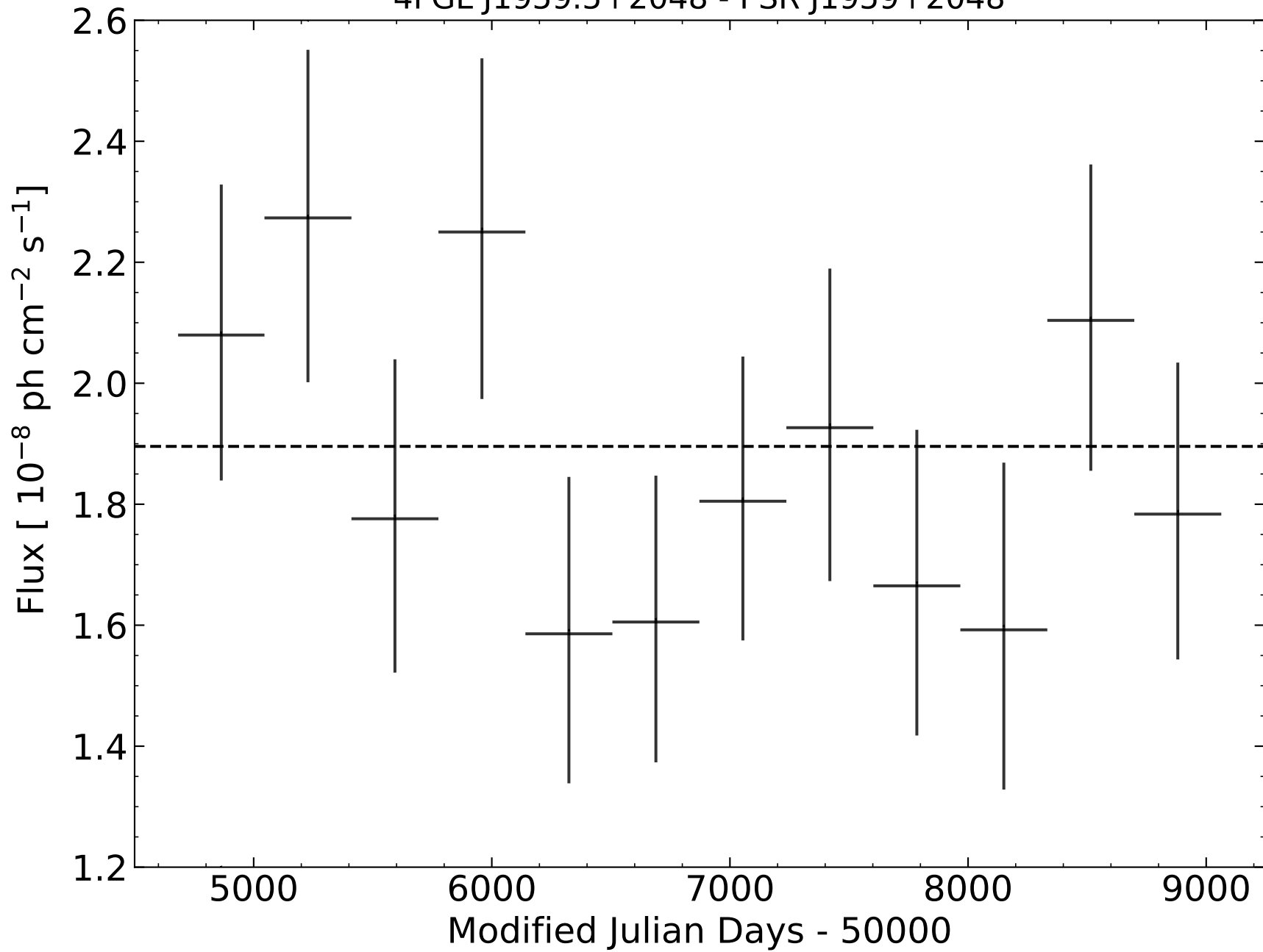
4FGL J1959.5+2048 - PSR J1959+2048
