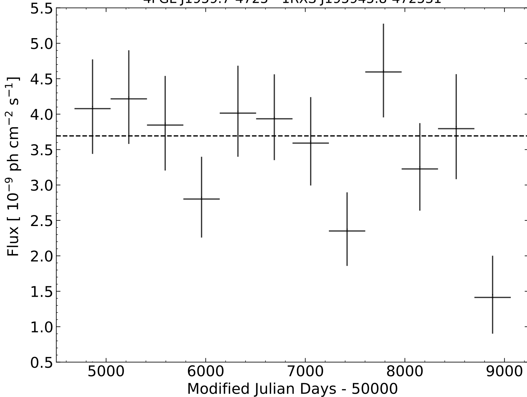
4FGL J1959.7-4725 - 1RXS J195945.8-472531
