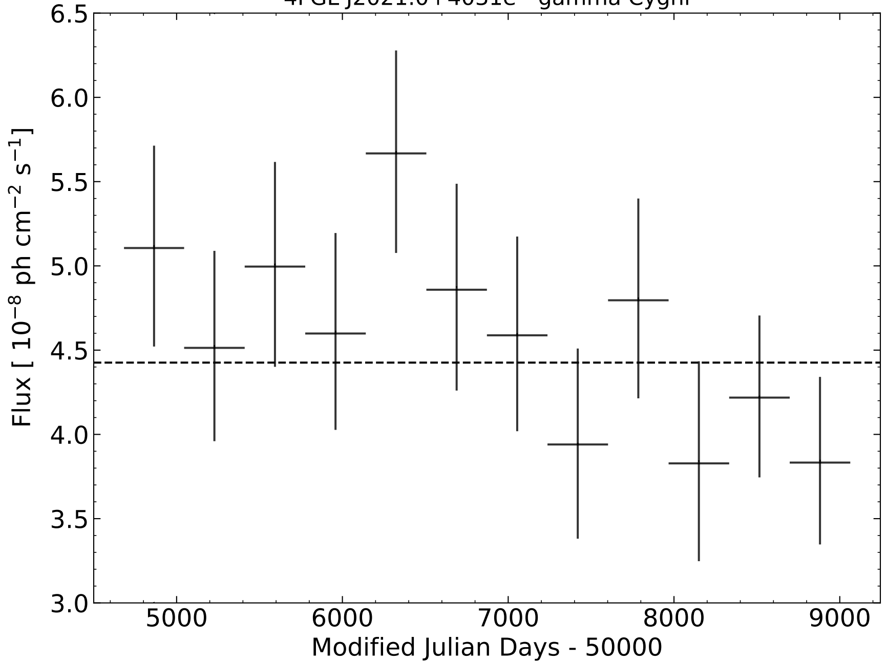
4FGL J2021.0+4031e - gamma Cygni
