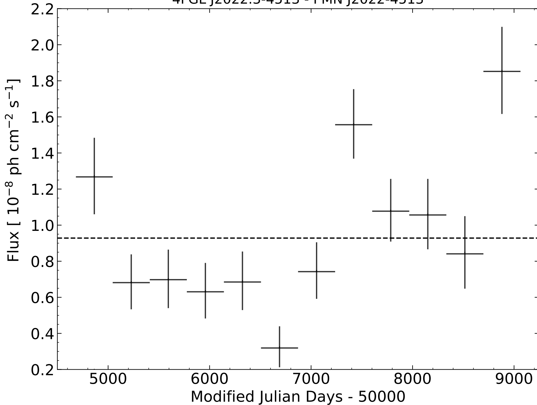
4FGL J2022.3-4513 - PMN J2022-4513
