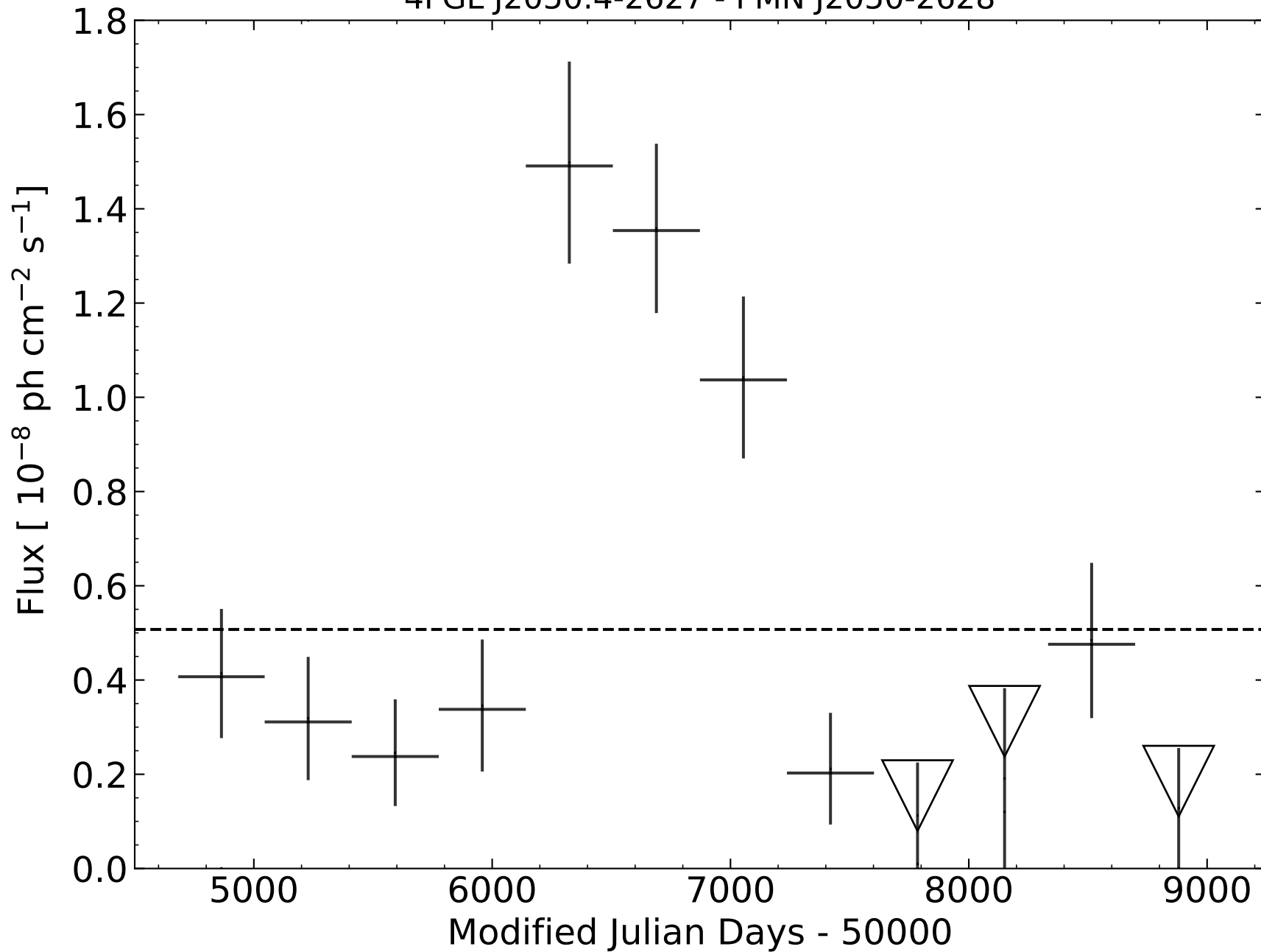
4FGL J2050.4-2627 - PMN J2050-2628
