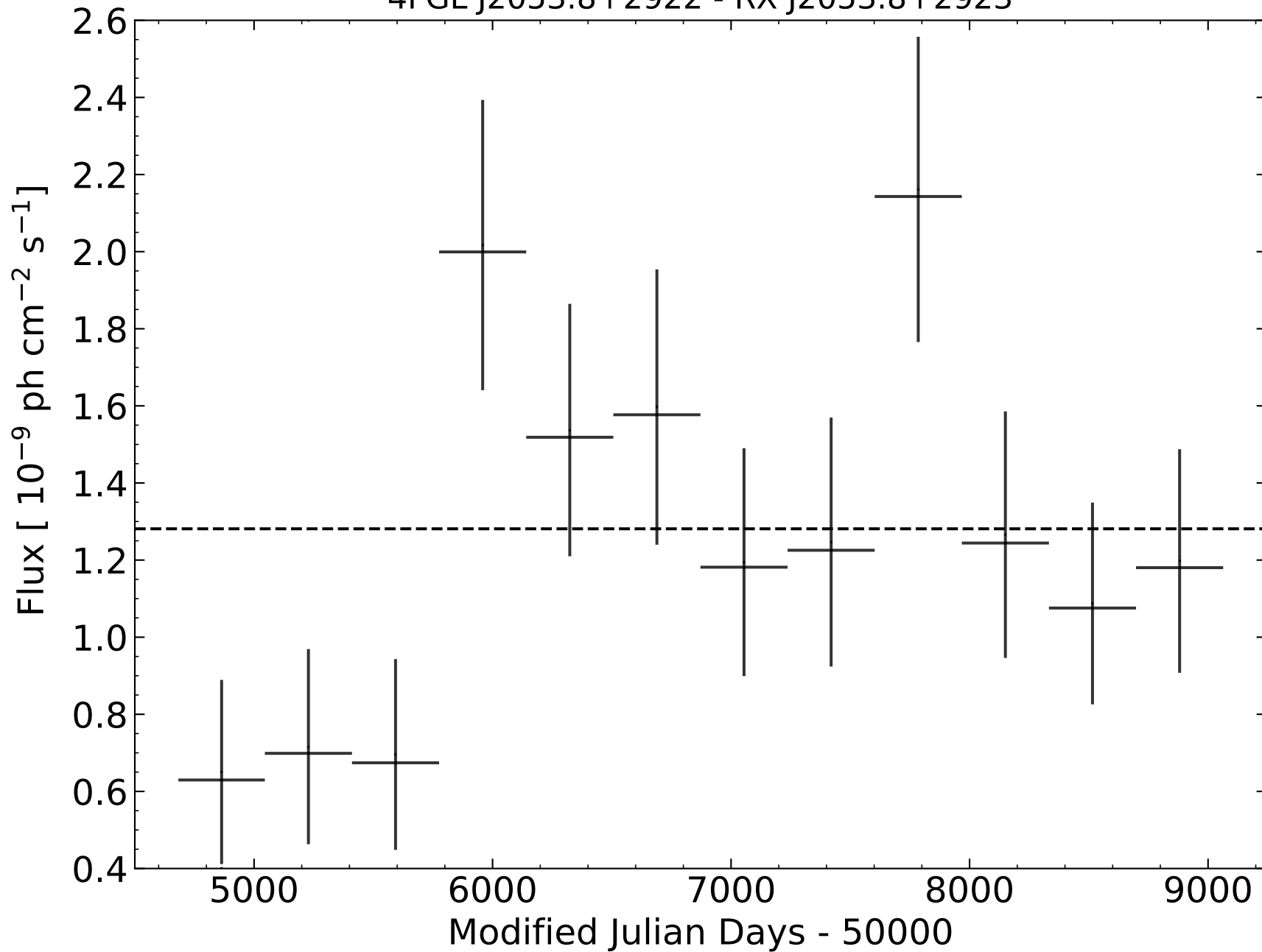
4FGL J2053.8+2922 - RX J2053.8+2923
