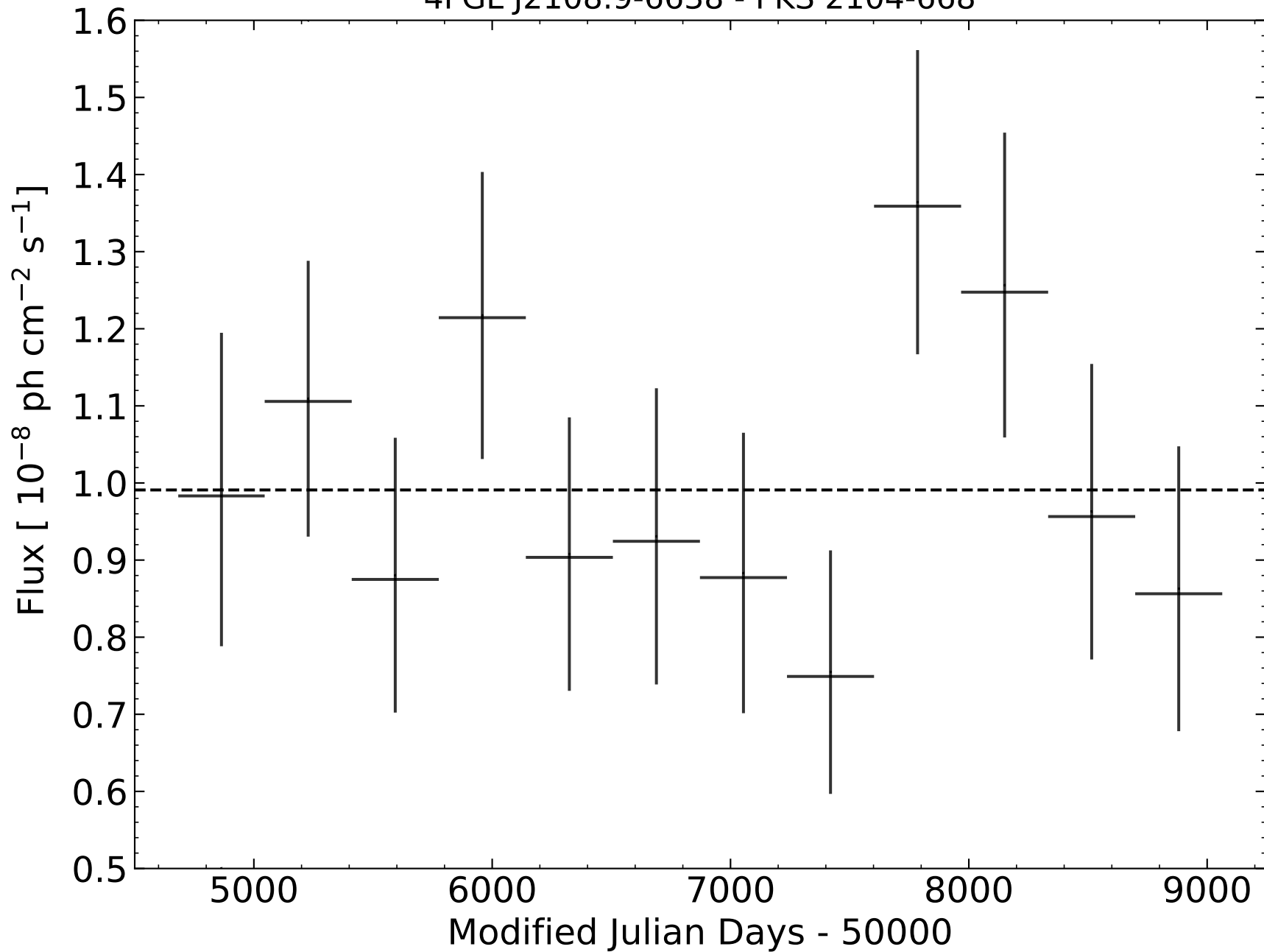
4FGL J2108.9-6638 - PKS 2104-668
