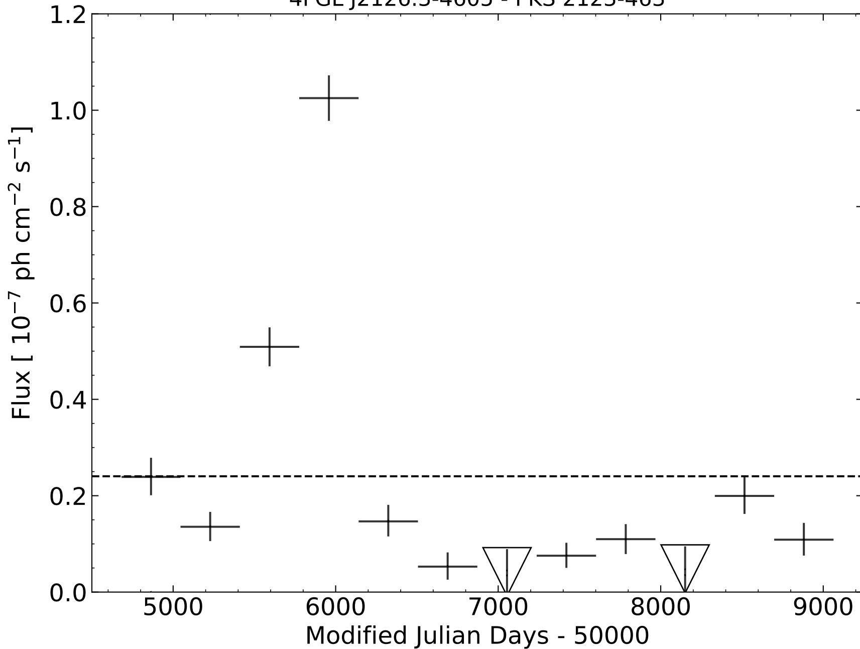
4FGL J2126.3-4605 - PKS 2123-463
