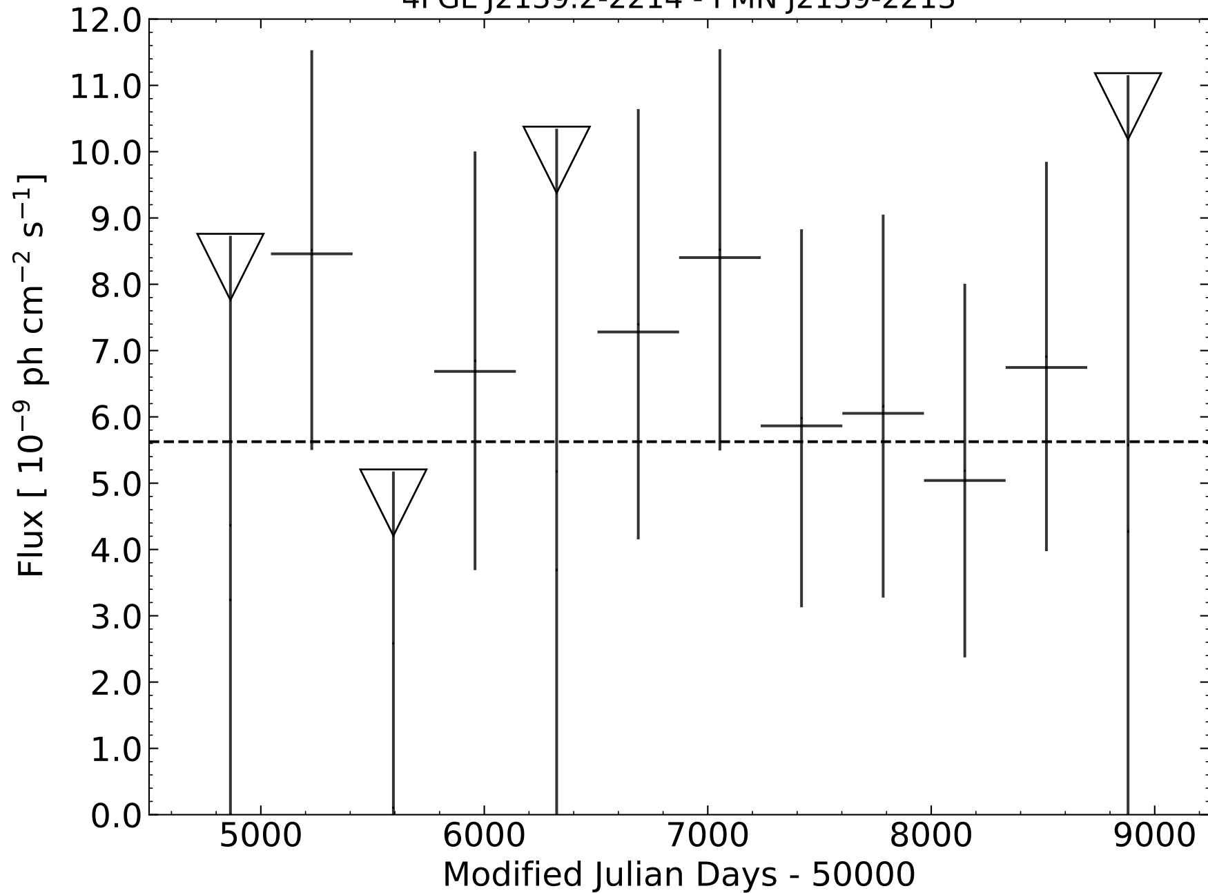
4FGL J2139.2-2214 - PMN J2139-2213
