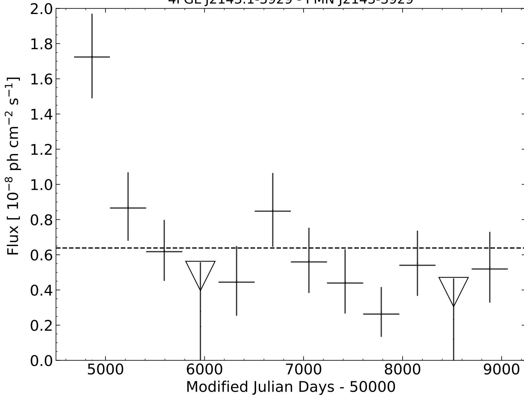
4FGL J2143.1-3929 - PMN J2143-3929
