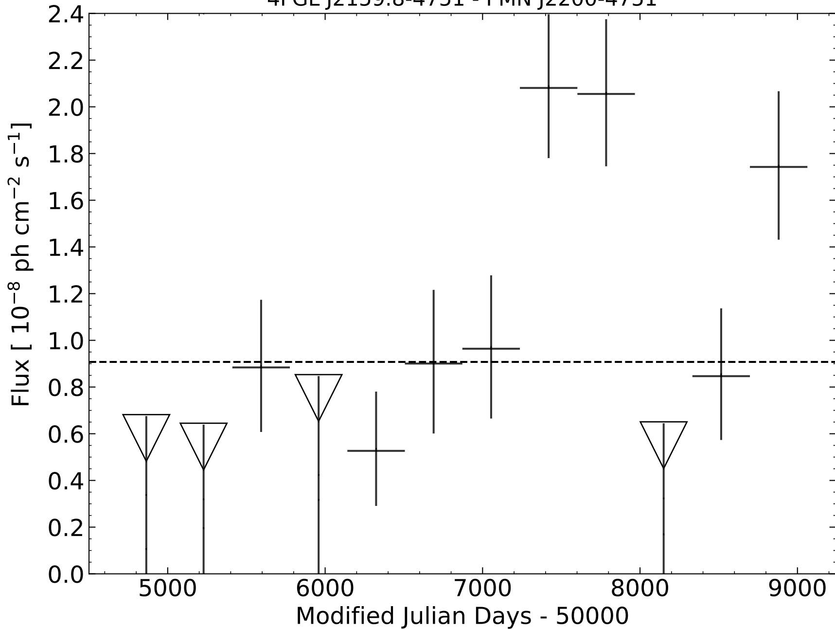
4FGL J2159.8-4751 - PMN J2200-4751
