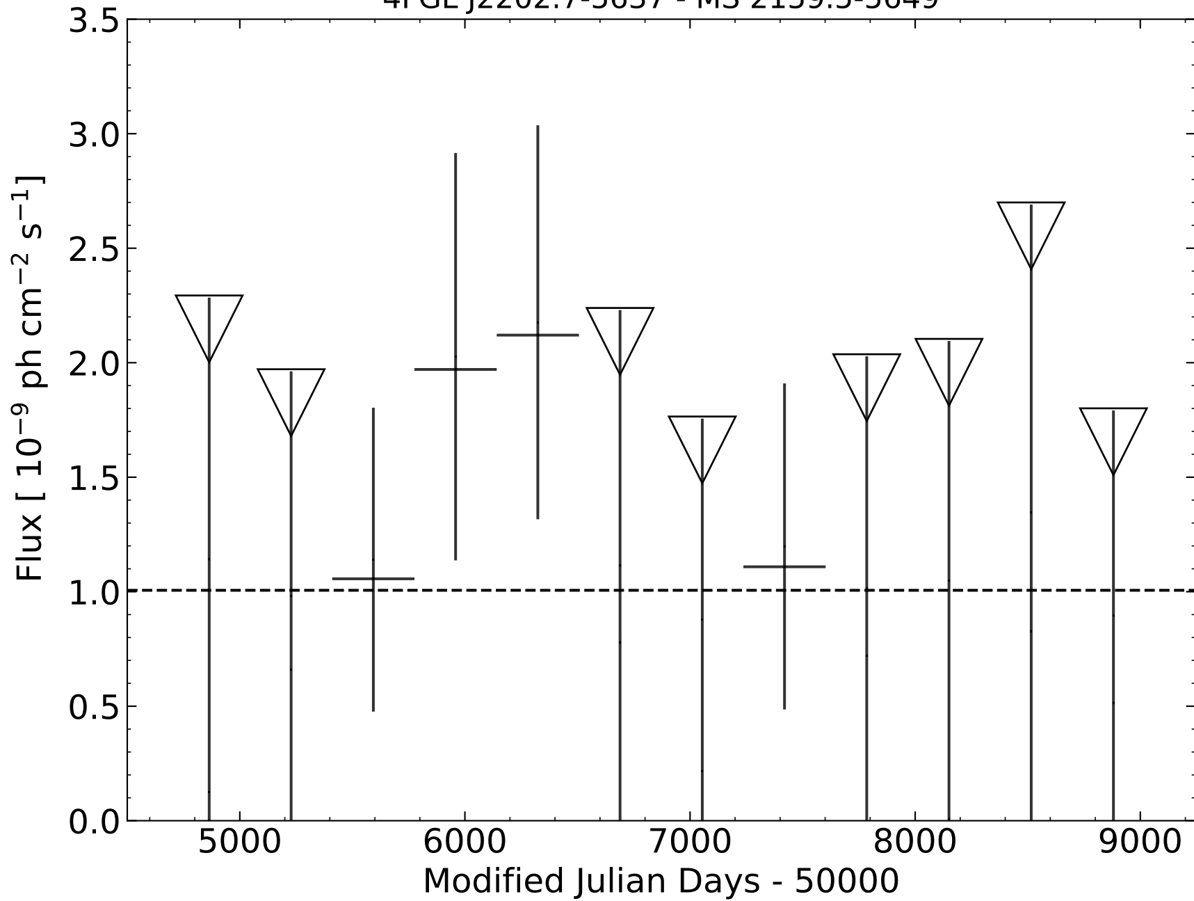
4FGL J2202.7-5637 - MS 2159.5-5649
