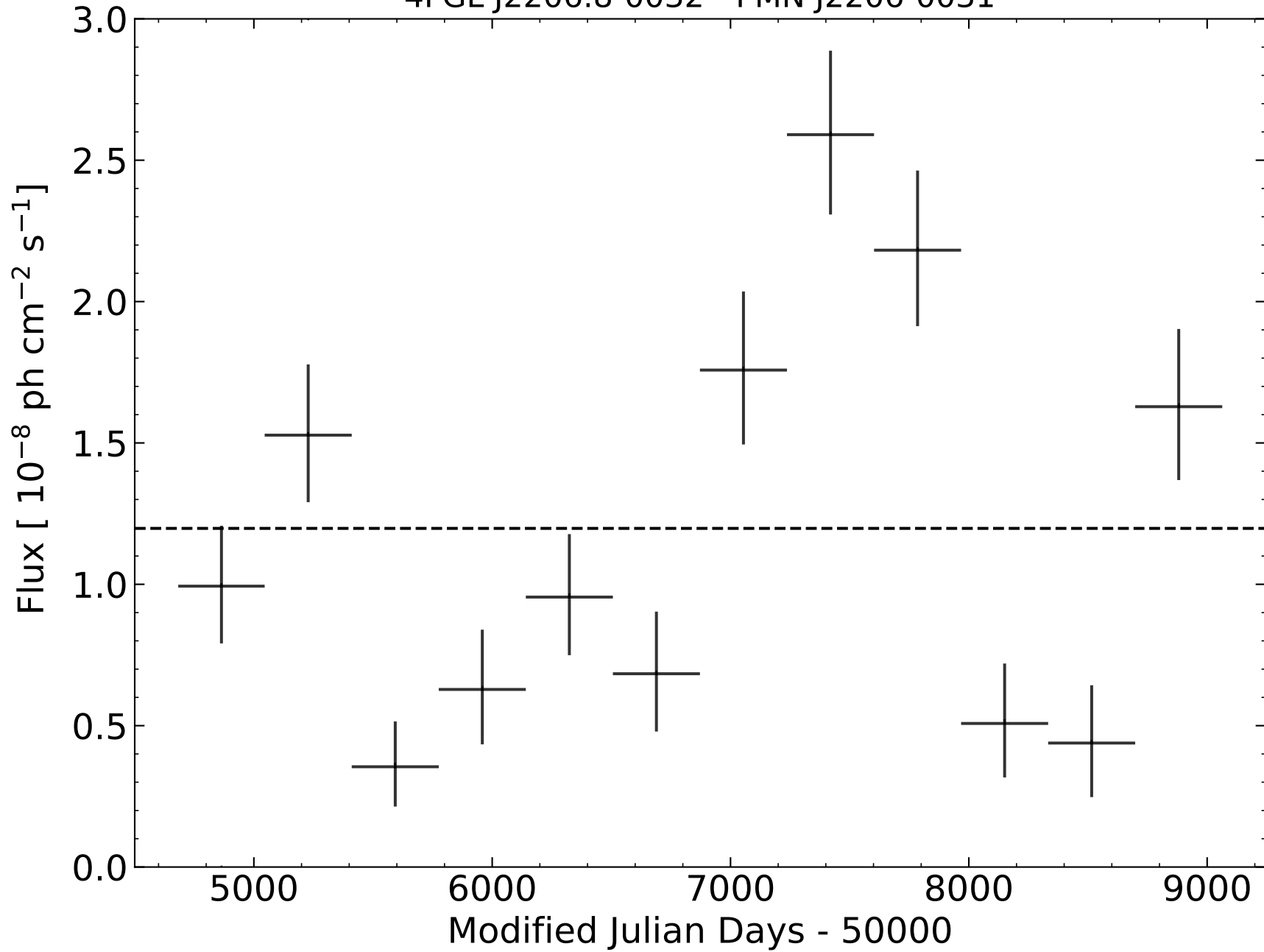
4FGL J2206.8-0032 - PMN J2206-0031
