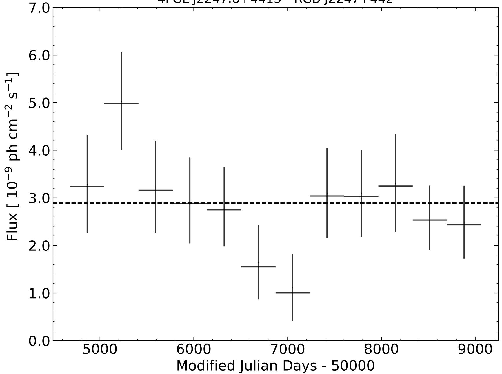
4FGL J2247.8+4413 - RGB J2247+442
