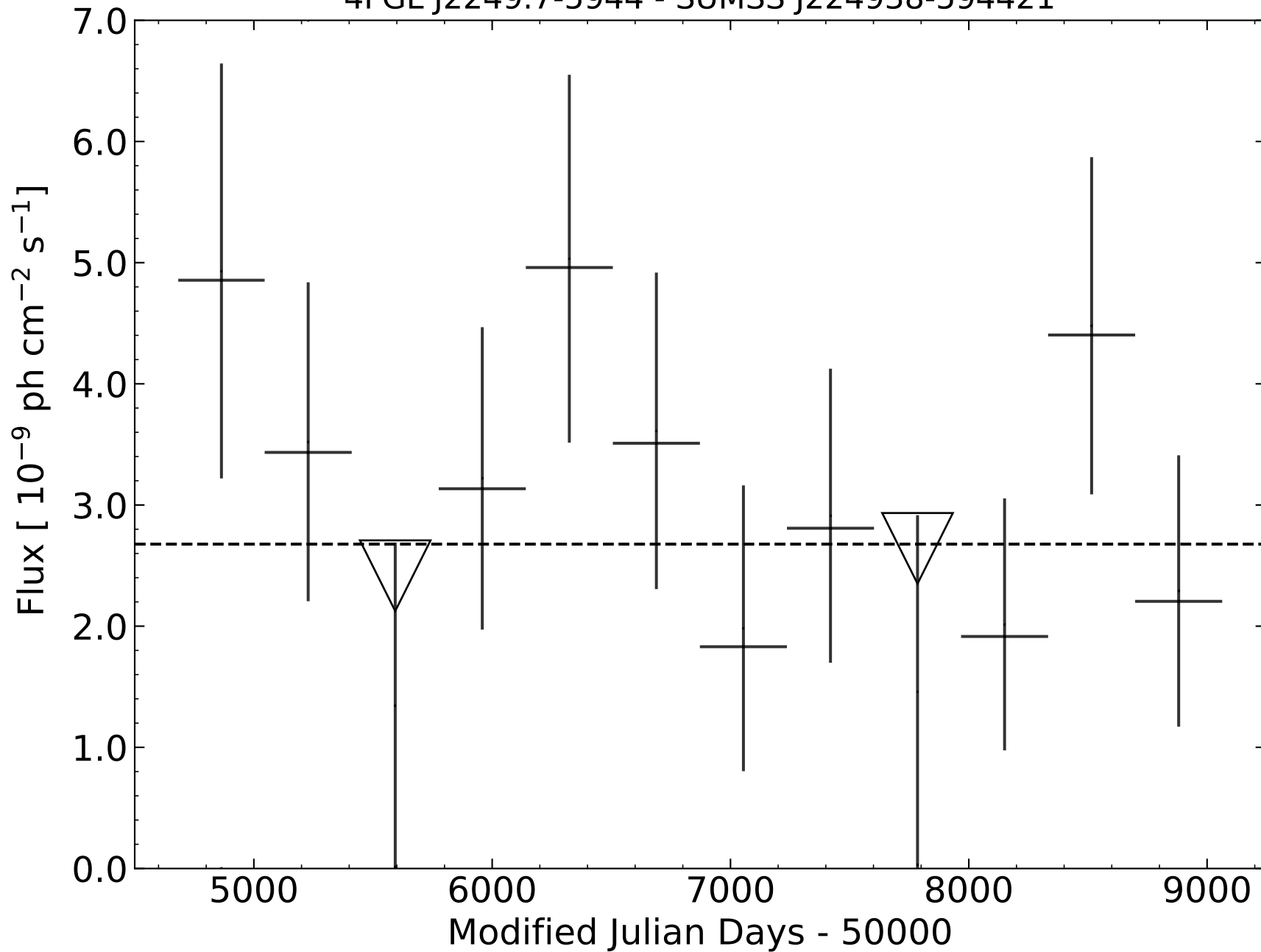
4FGL J2249.7-5944 - SUMSS J224938-594421
