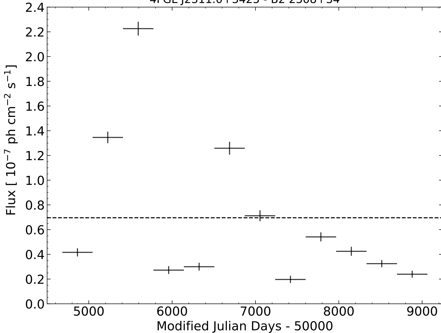
4FGL J2311.0+3425 - B2 2308+34
