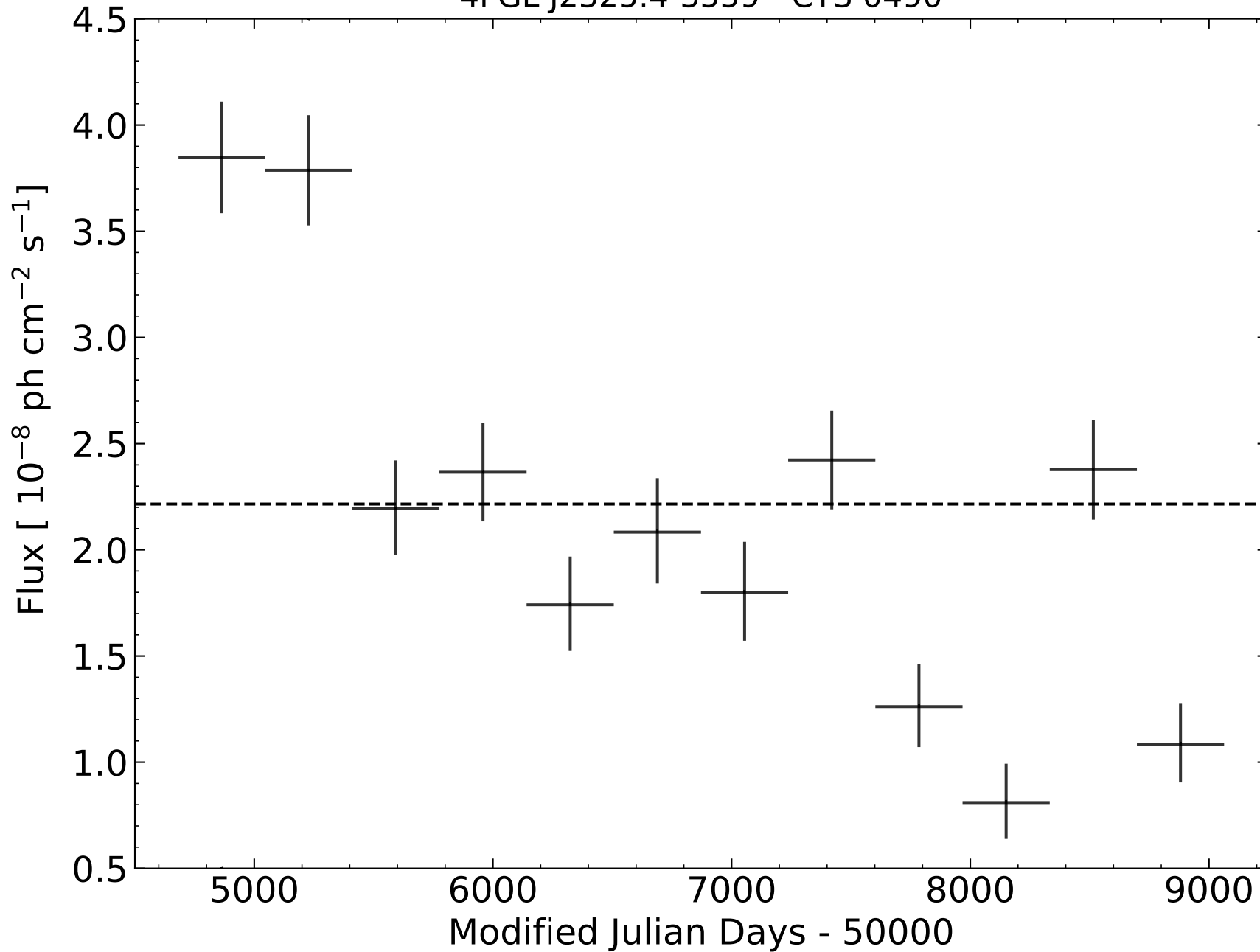
4FGL J2325.4-3559 - CTS 0490
