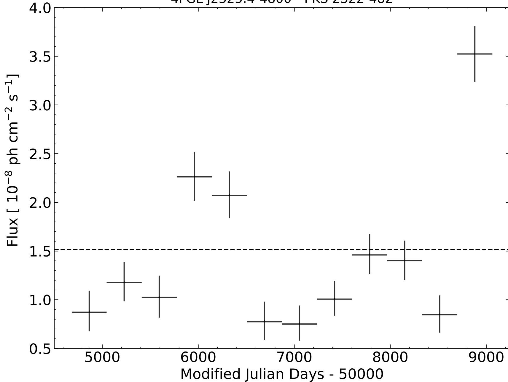
4FGL J2325.4-4800 - PKS 2322-482
