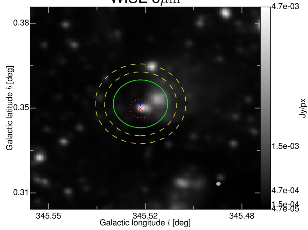
WISE 3 \mu\text{m}
