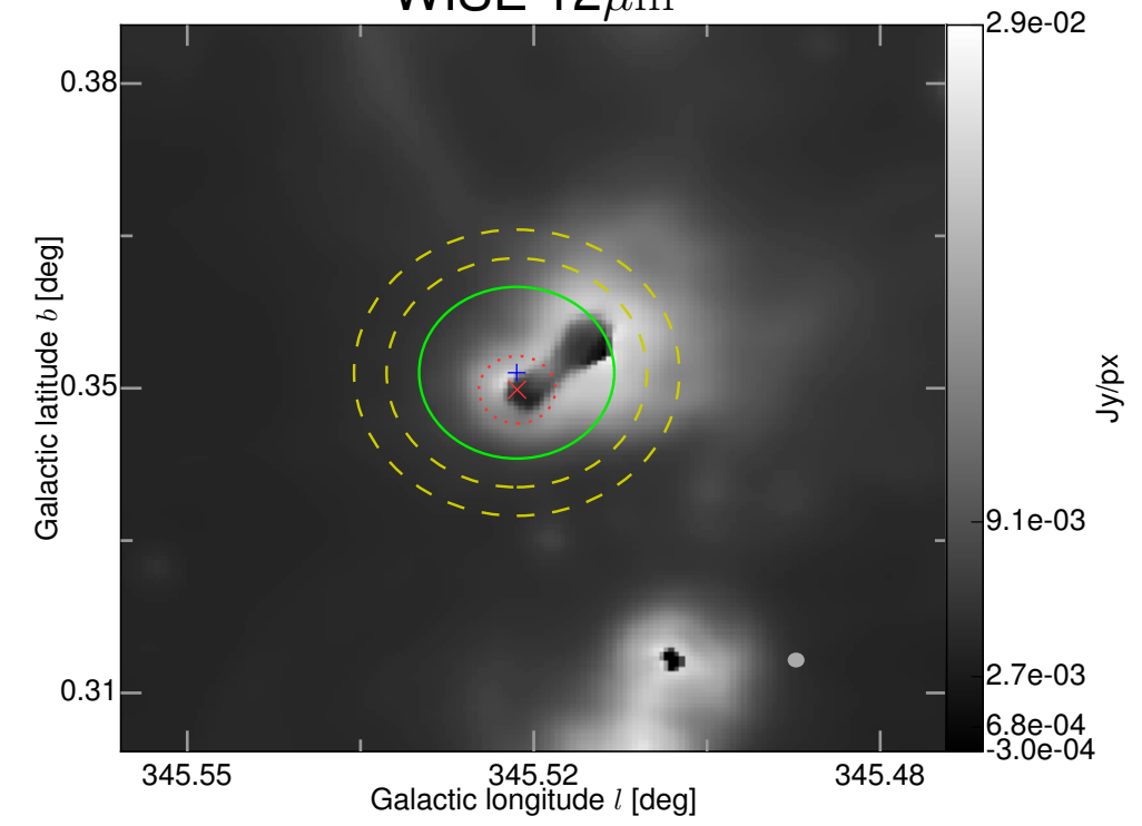
WISE 12 \mu\text{m}
