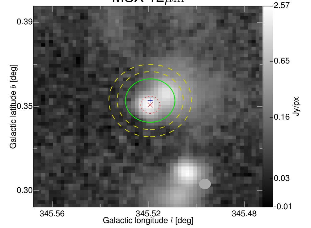
MSX 12 \mu\text{m}
