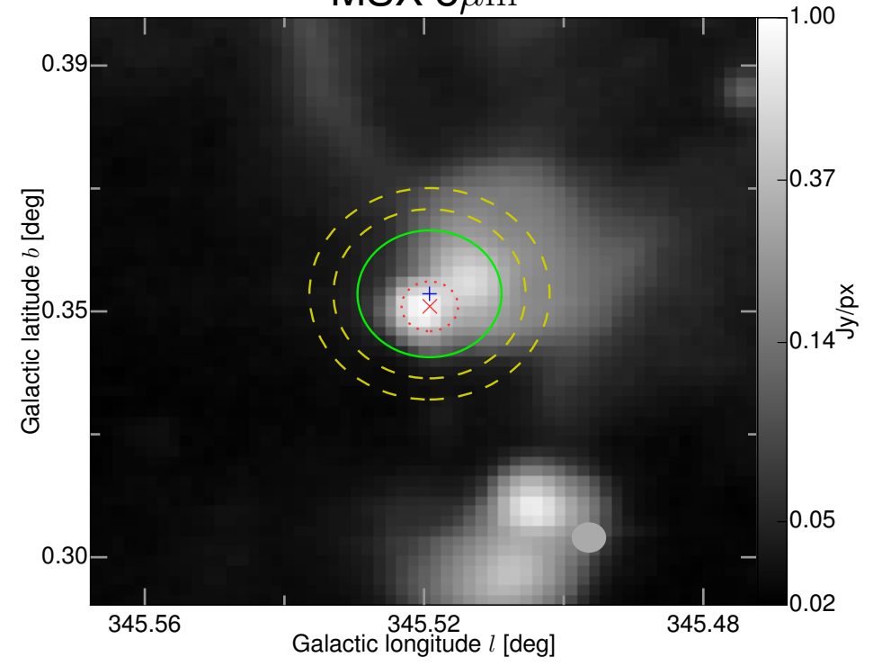
MSX 8 \mu\text{m}
