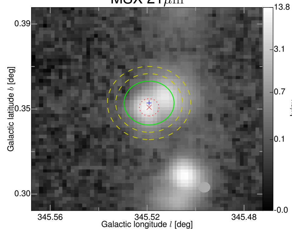
MSX 21 \mu\text{m}
