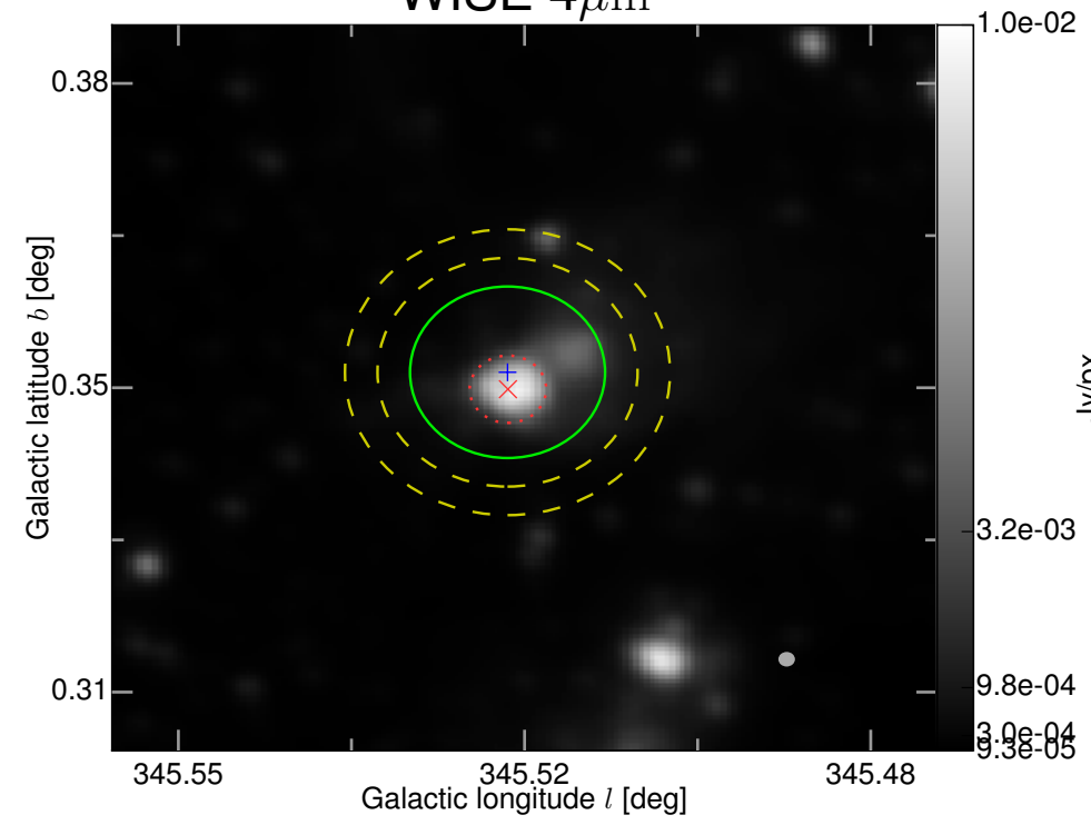
WISE 4 \mu\text{m}
