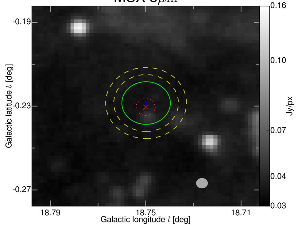
MSX 8 \mu\text{m}
