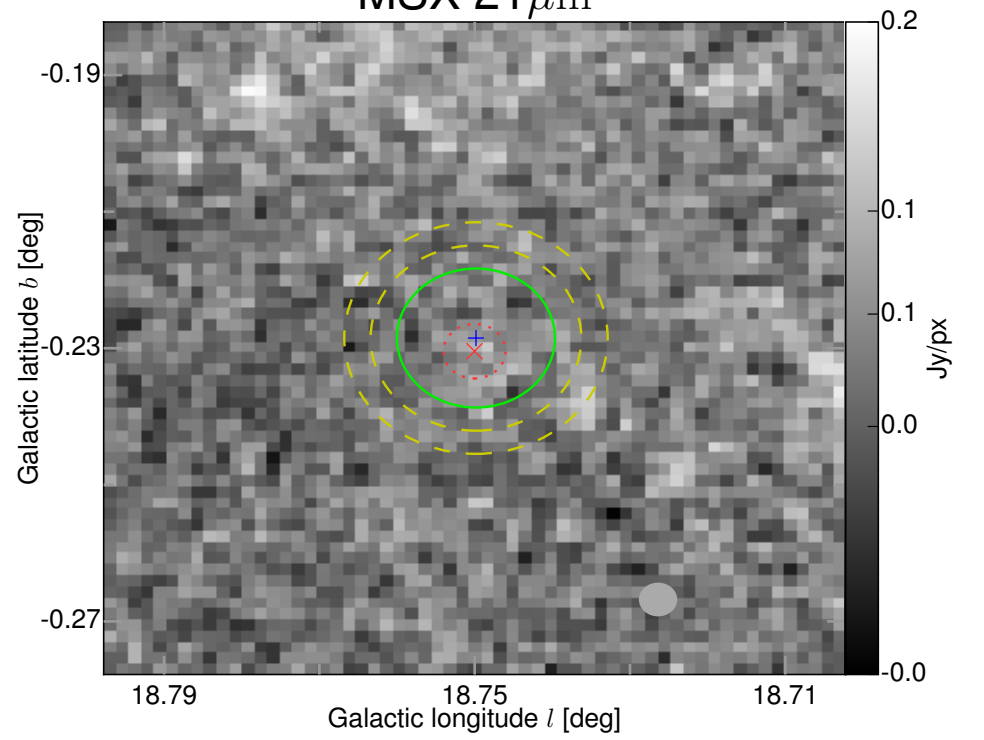
MSX 21 \mu\text{m}
