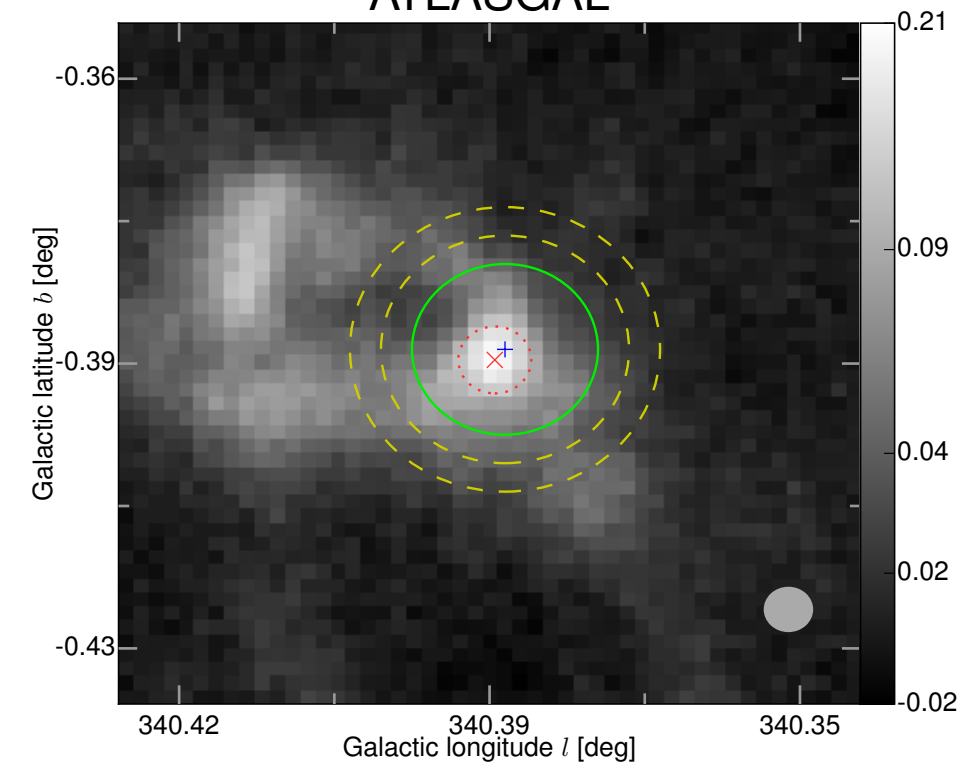
ATLASGAL
