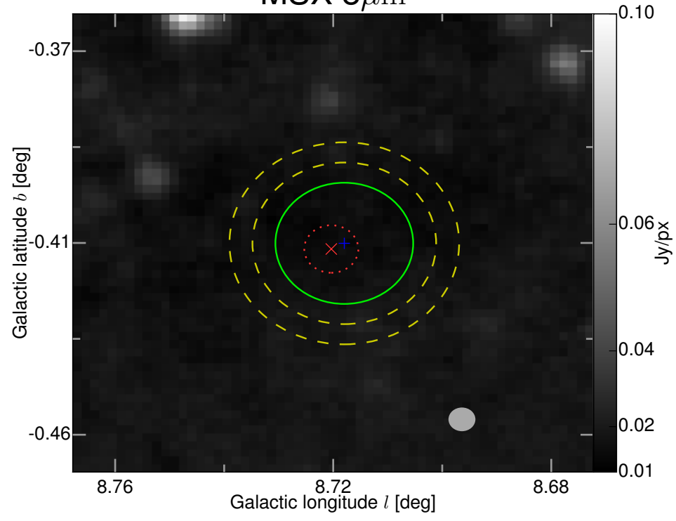
MSX 8\mu\text{m}
