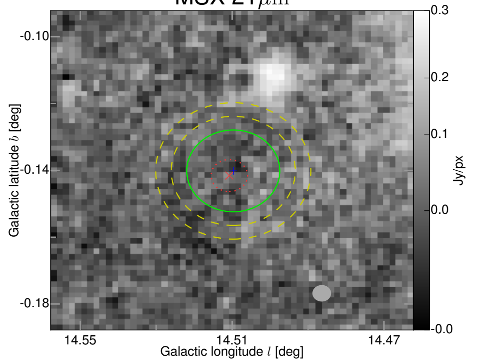
MSX 21 \mu\text{m}
