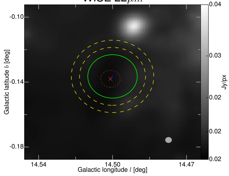
WISE 22 \mu\text{m}
