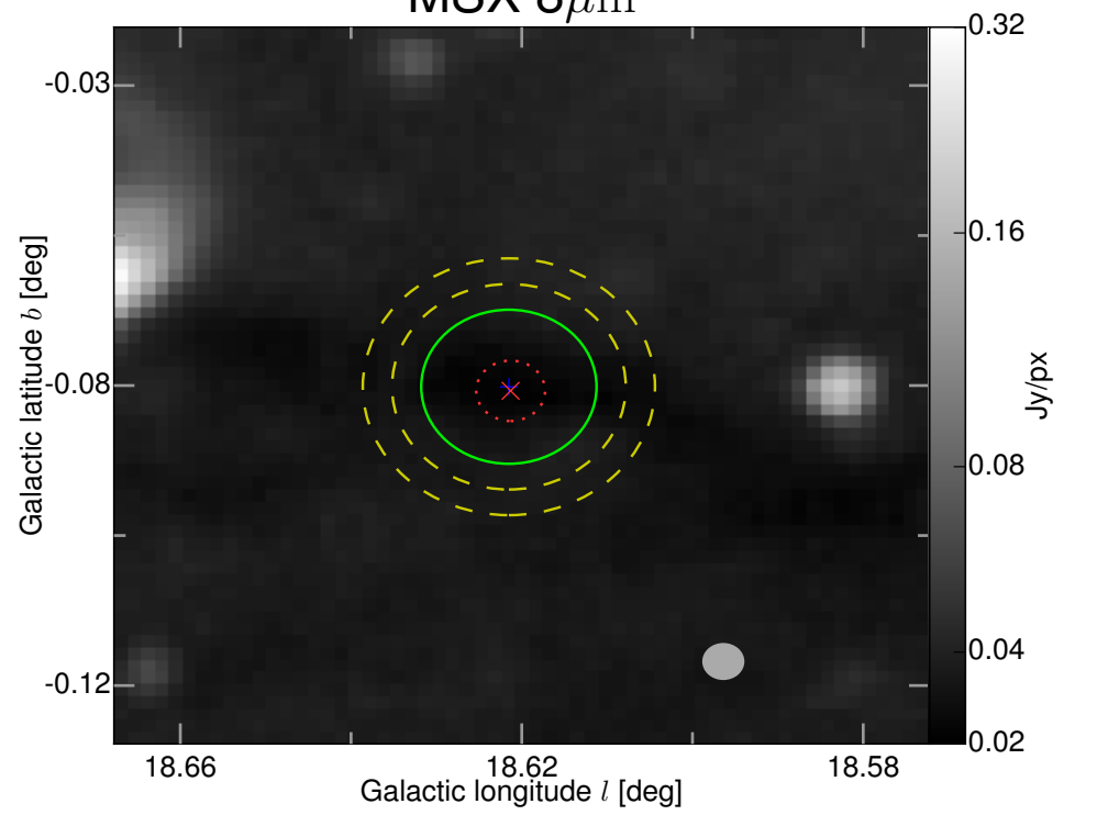
MSX 8\mu\text{m}
