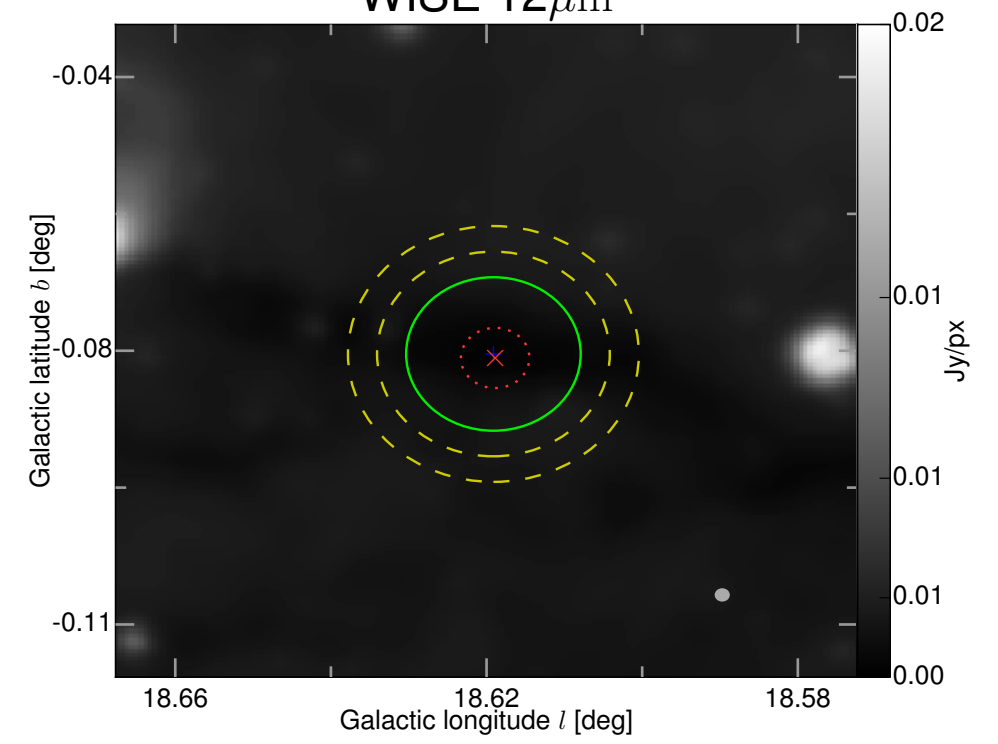
WISE 12\mu\text{m}
