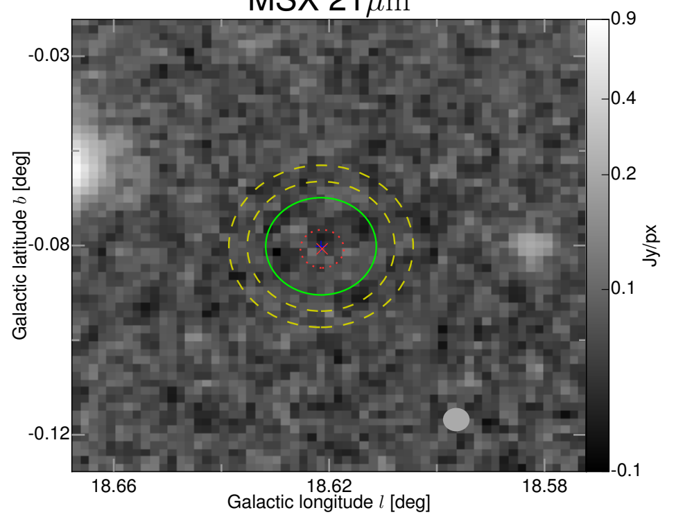
MSX 21\mu\text{m}
