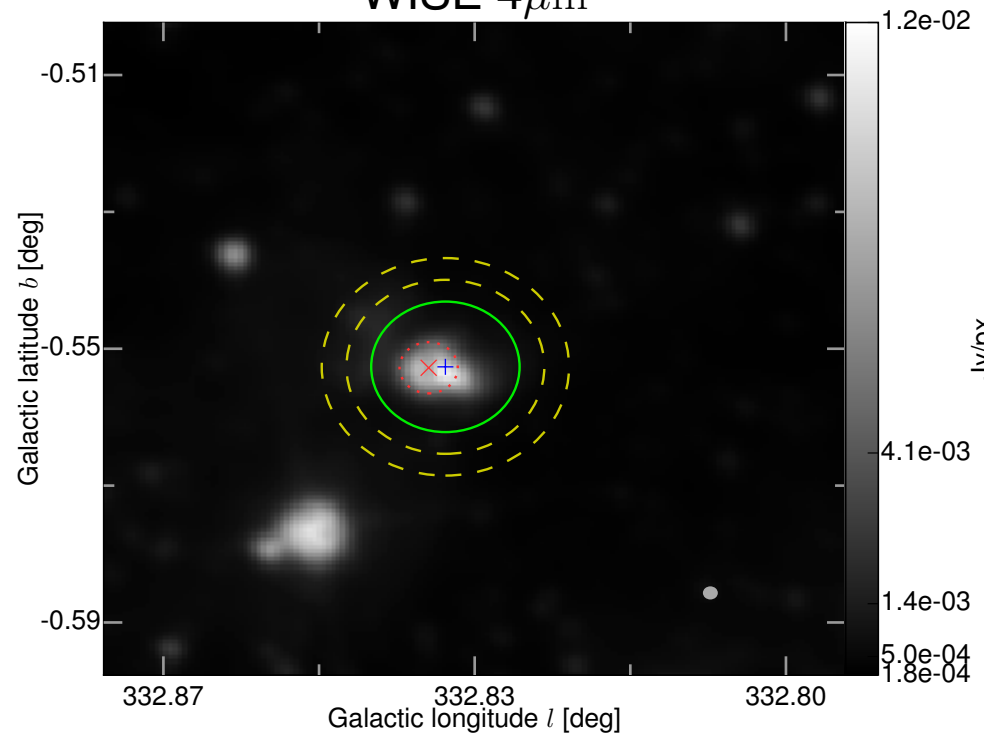
WISE 4 \mu\text{m}
