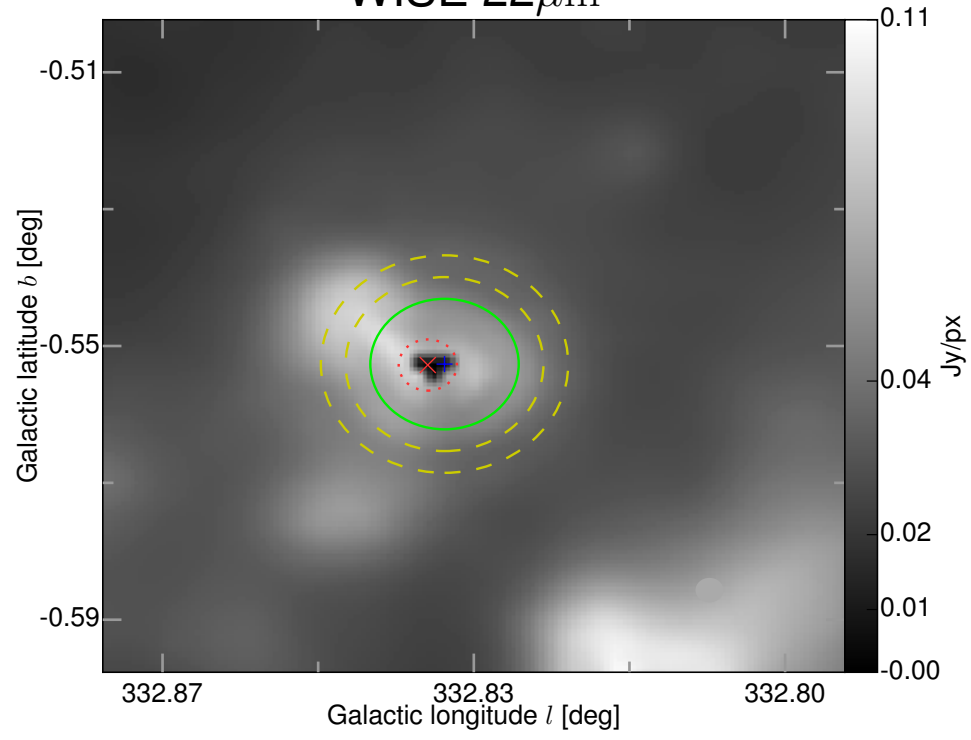
WISE 22 \mu\text{m}
