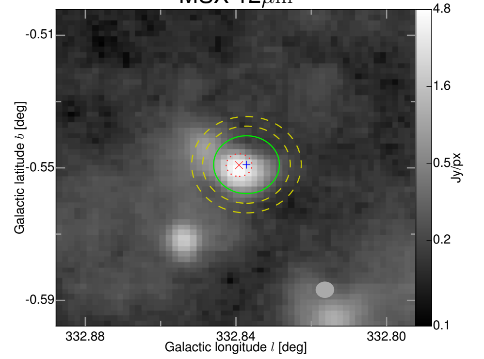
MSX 12 \mu\text{m}
