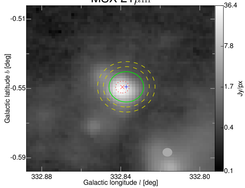
MSX 21 \mu\text{m}
