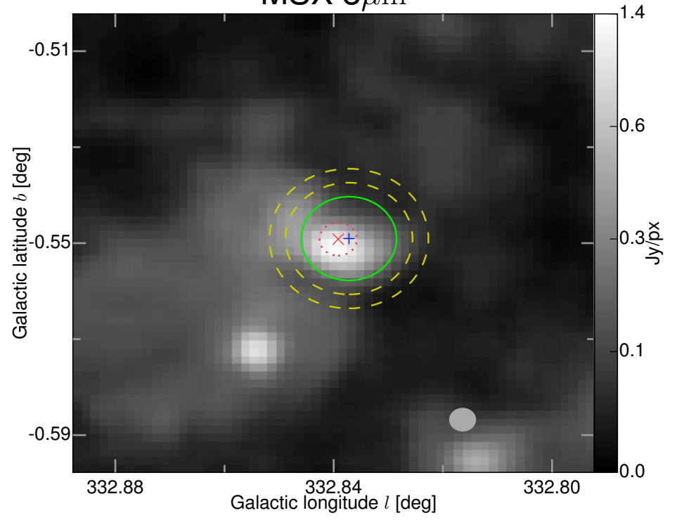
MSX 8 \mu\text{m}
