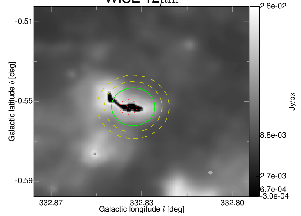
WISE 12 \mu\text{m}
