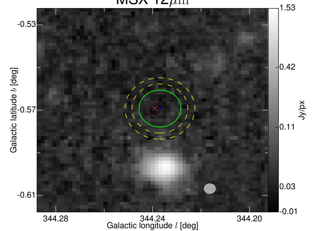
MSX 12 \mu\text{m}
