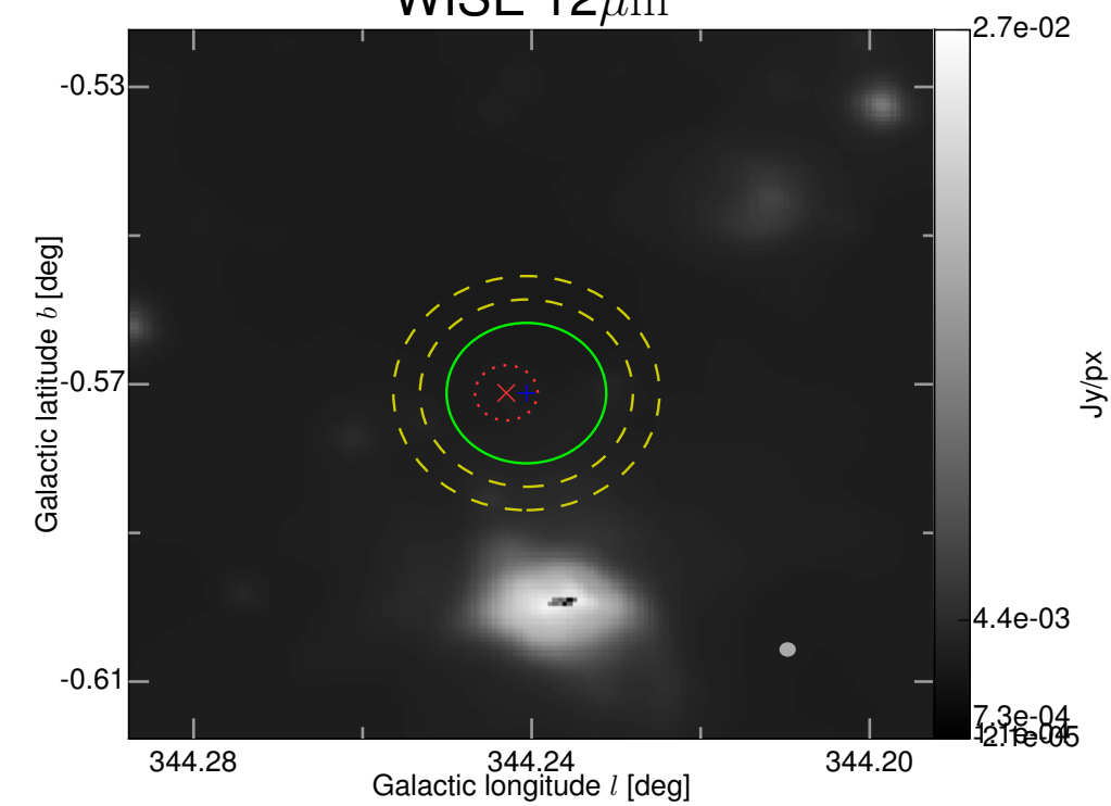
WISE 12 \mu\text{m}
