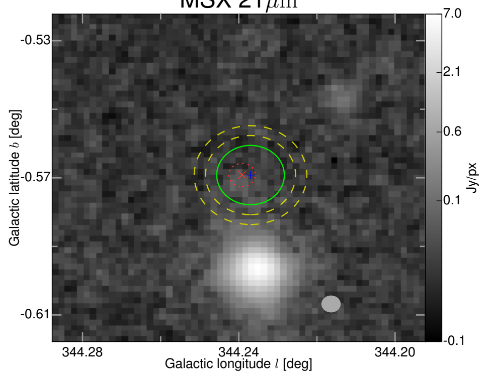
MSX 21 \mu\text{m}
