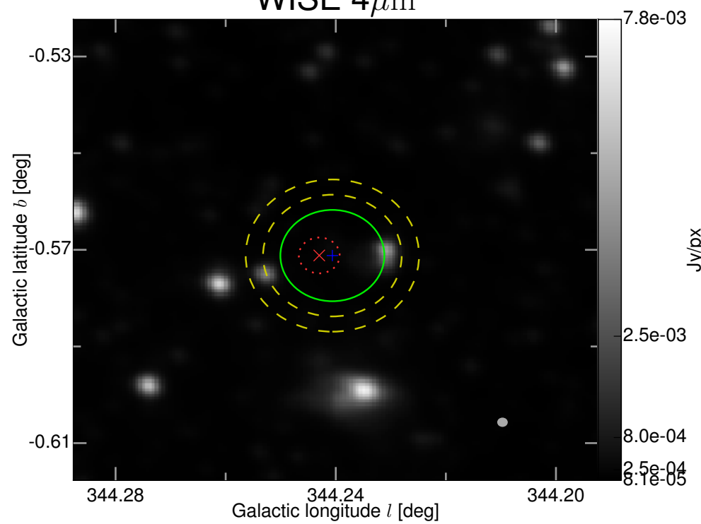
WISE 4 \mu\text{m}
