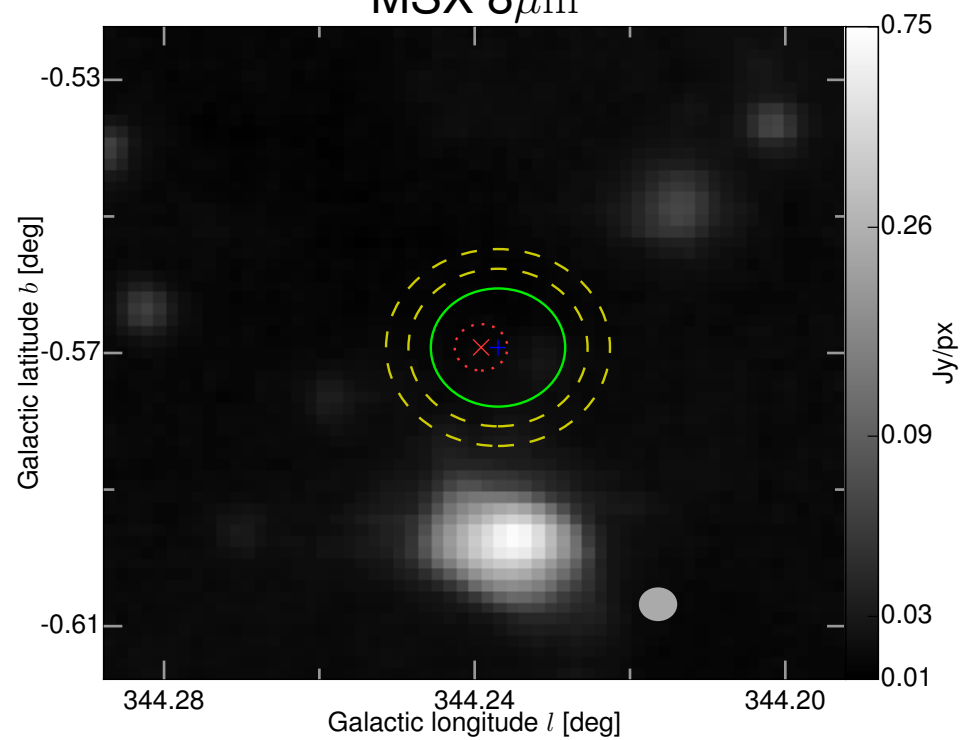
MSX 8 \mu\text{m}
