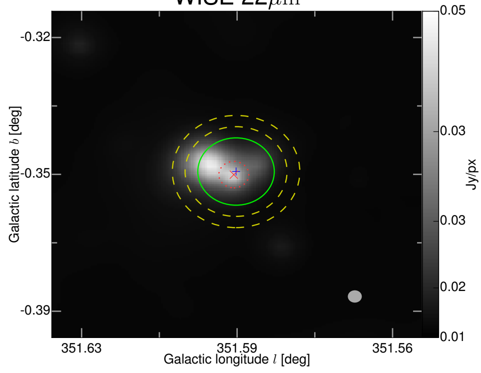
WISE 22 \mu\text{m}
