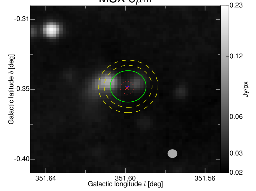
MSX 8 \mu\text{m}
