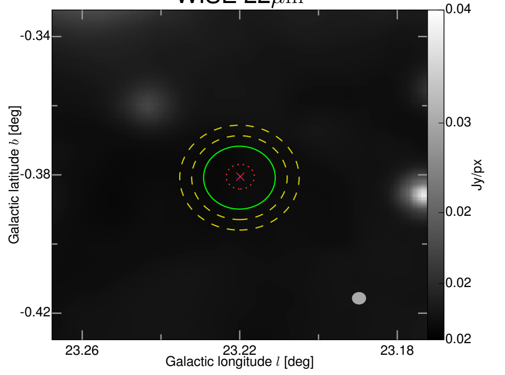
WISE 22 \mu\text{m}
