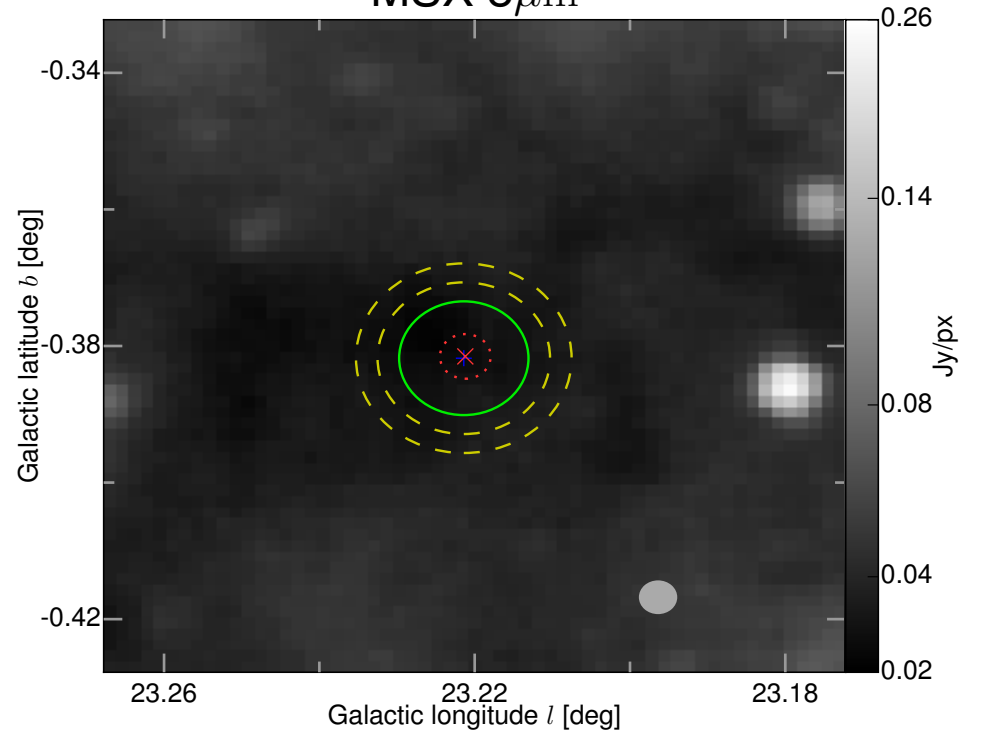
MSX 8 \mu\text{m}
