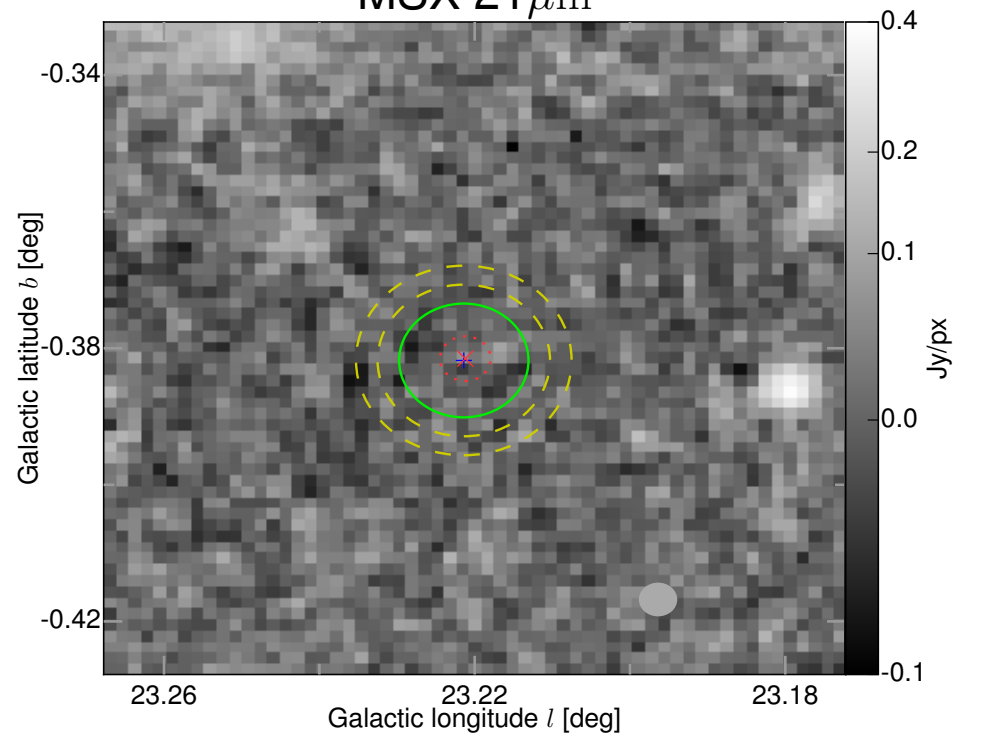
MSX 21 \mu\text{m}
