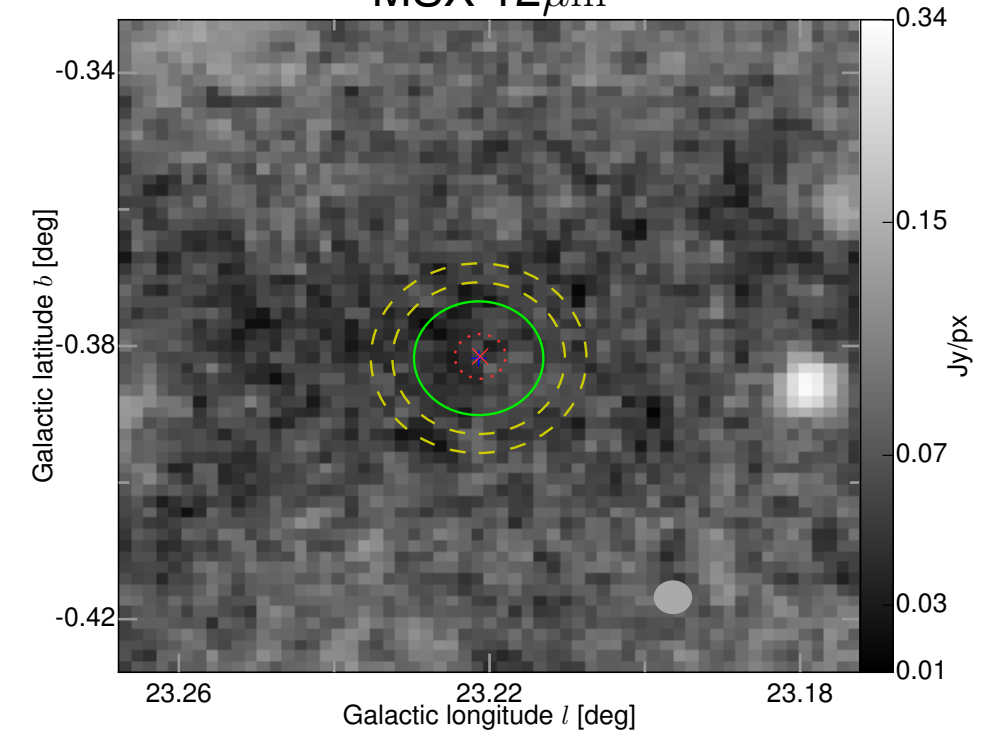
MSX 12 \mu\text{m}
