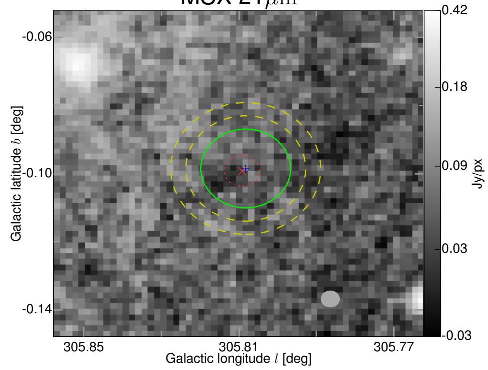
MSX 21 \mu\text{m}
