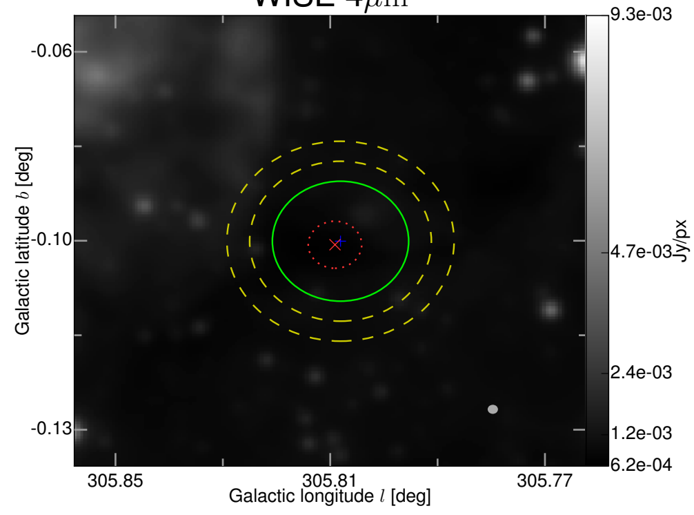
WISE 4 \mu\text{m}
