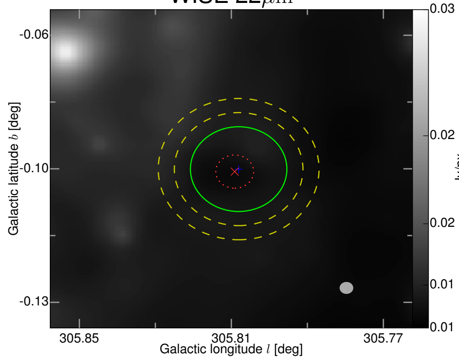
WISE 22 \mu\text{m}
