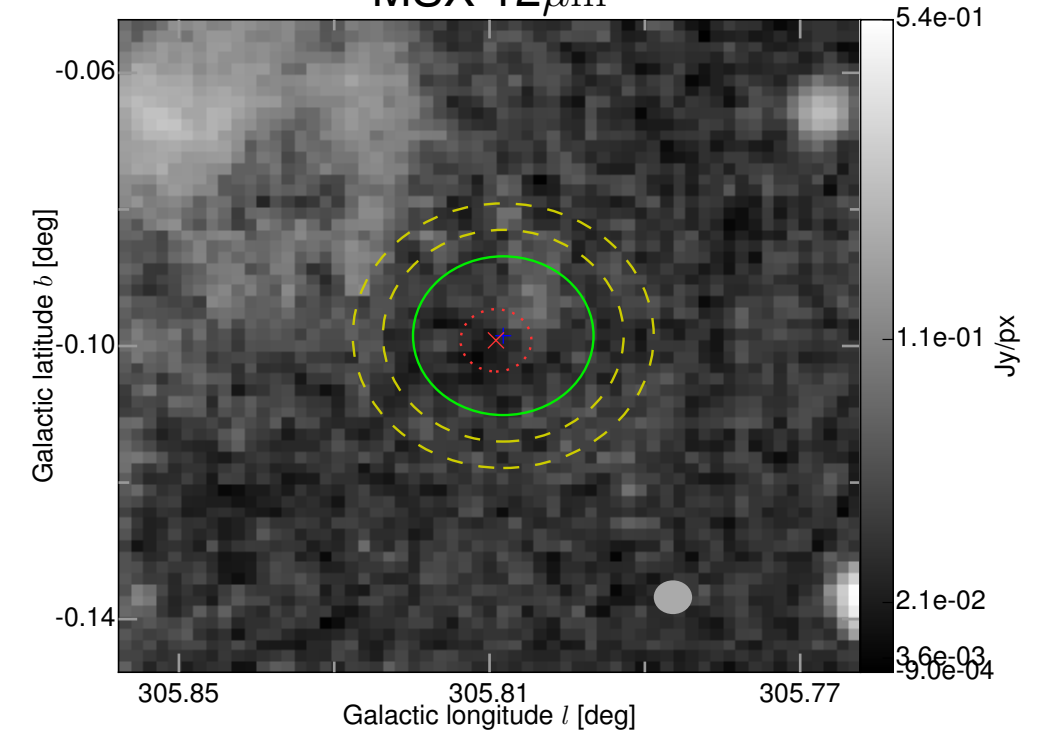
MSX 12 \mu\text{m}
