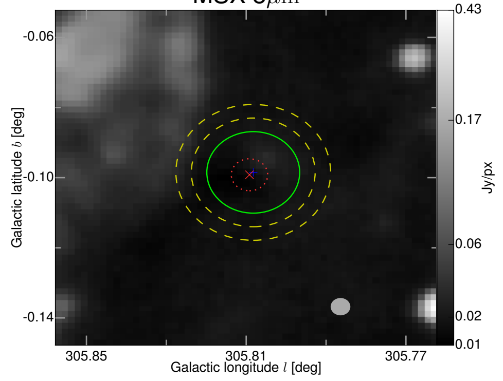
MSX 8 \mu\text{m}
