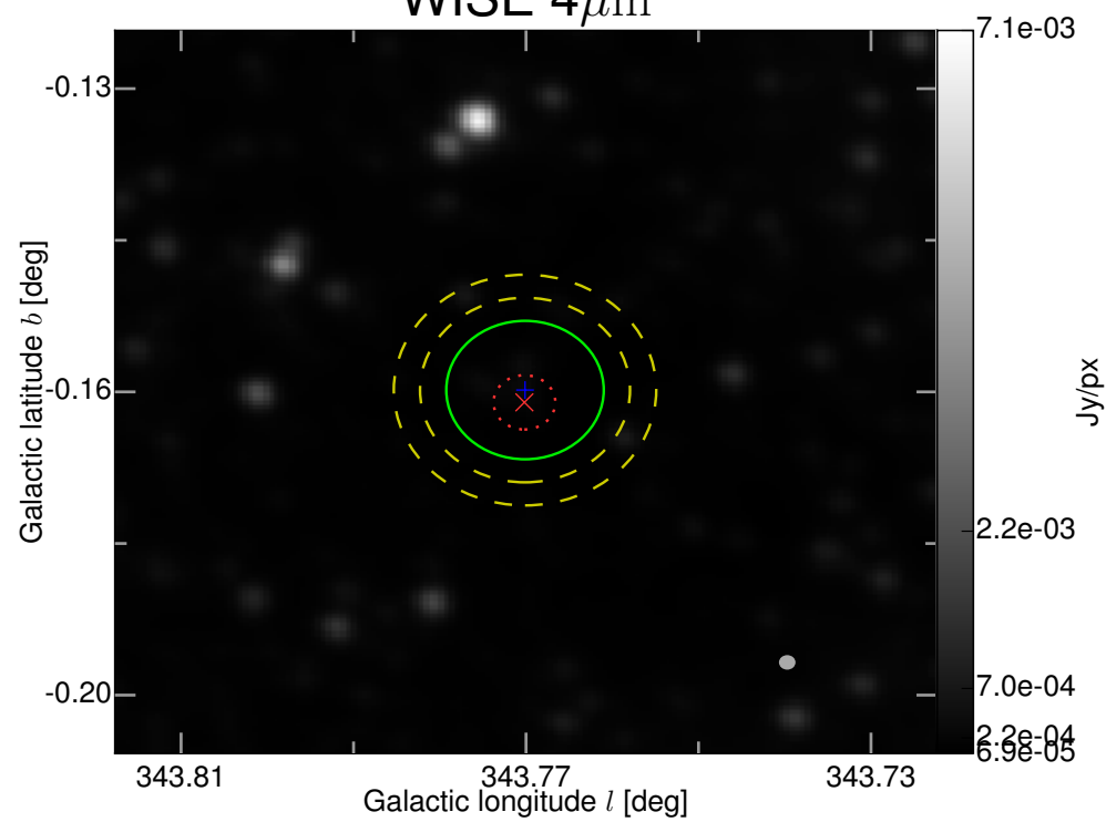
WISE 4\mu\text{m}
