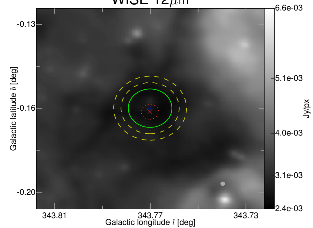
WISE 12\mu\text{m}
