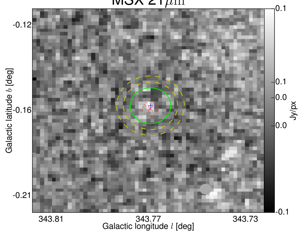
MSX 21\mu\text{m}
