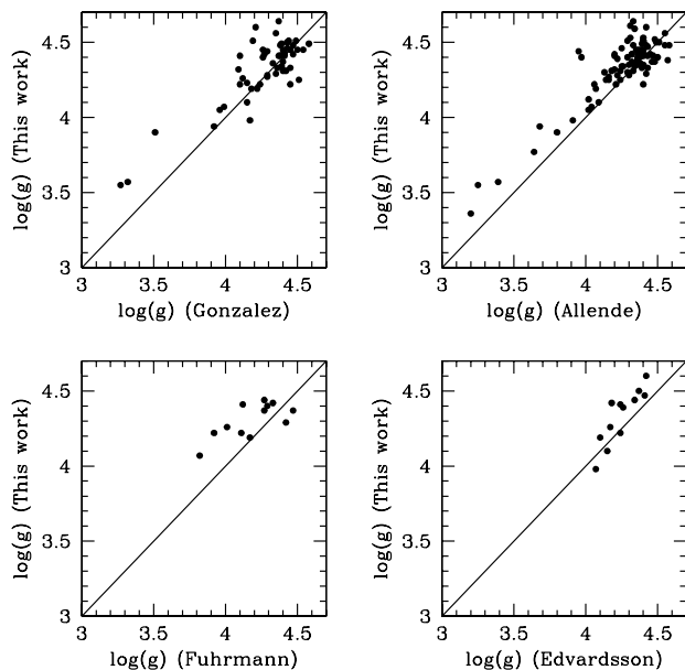
Fig. 2. Comparison of the spectroscopic \log g values derived in this work with the ones obtained by other authors for the same stars. The solid line represents a 1:1 relation. See text for more details.
