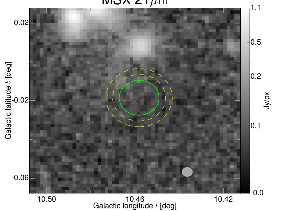
MSX 21\mu\text{m}
