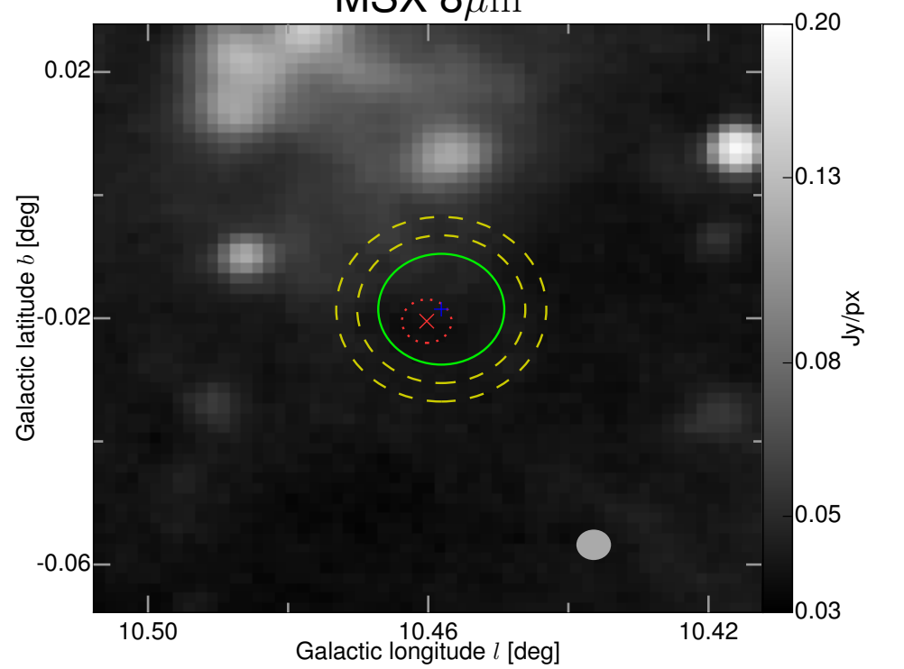
MSX 8\mu\text{m}
