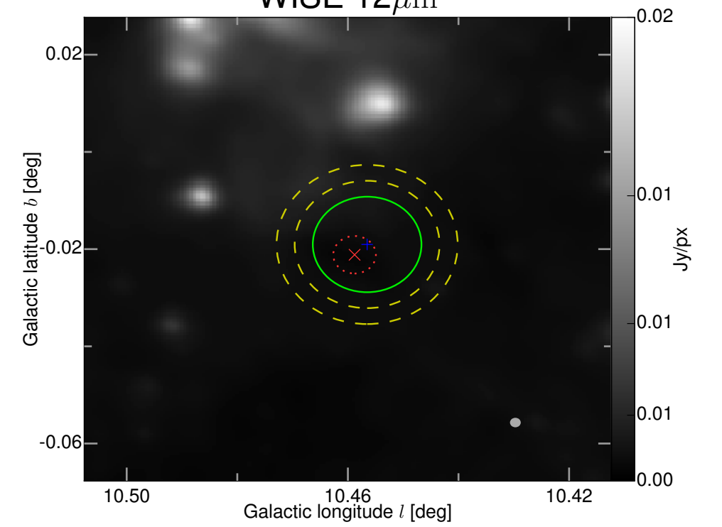
WISE 12\mu\text{m}
