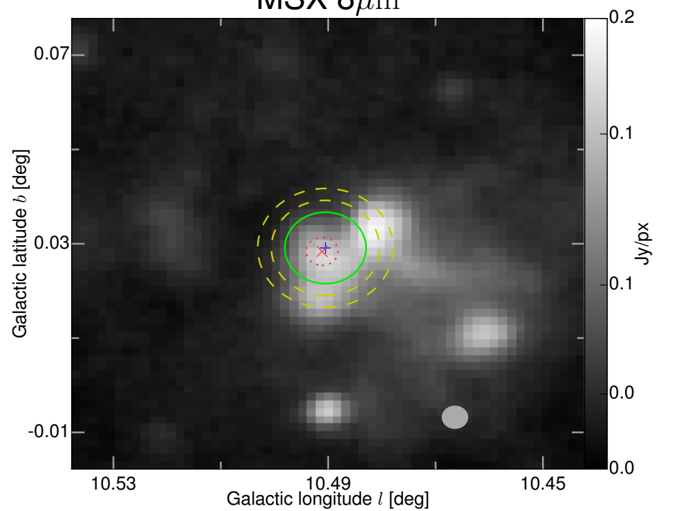
MSX 8\mu\text{m}
