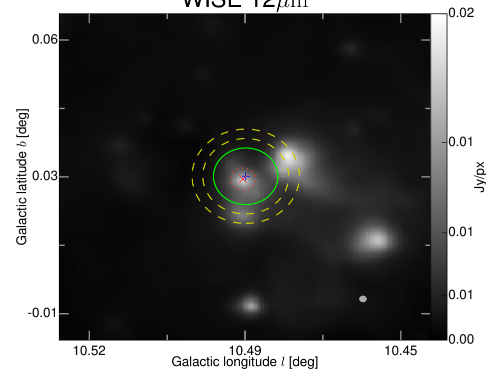
WISE 12\mu\text{m}
