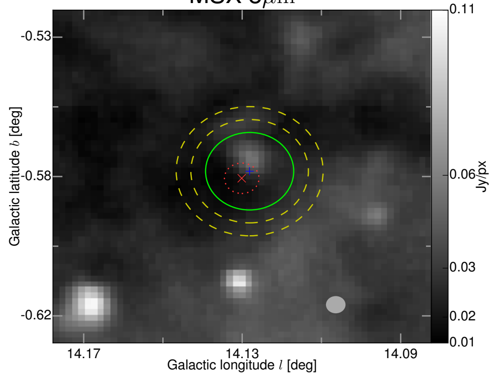
MSX 8\mu\text{m}
