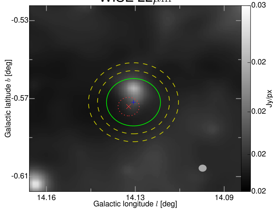
WISE 22\mu\text{m}
