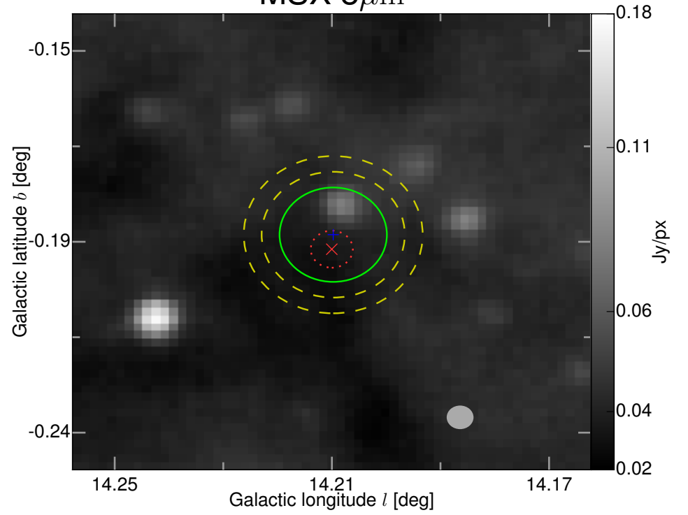
MSX 8\mu\text{m}
