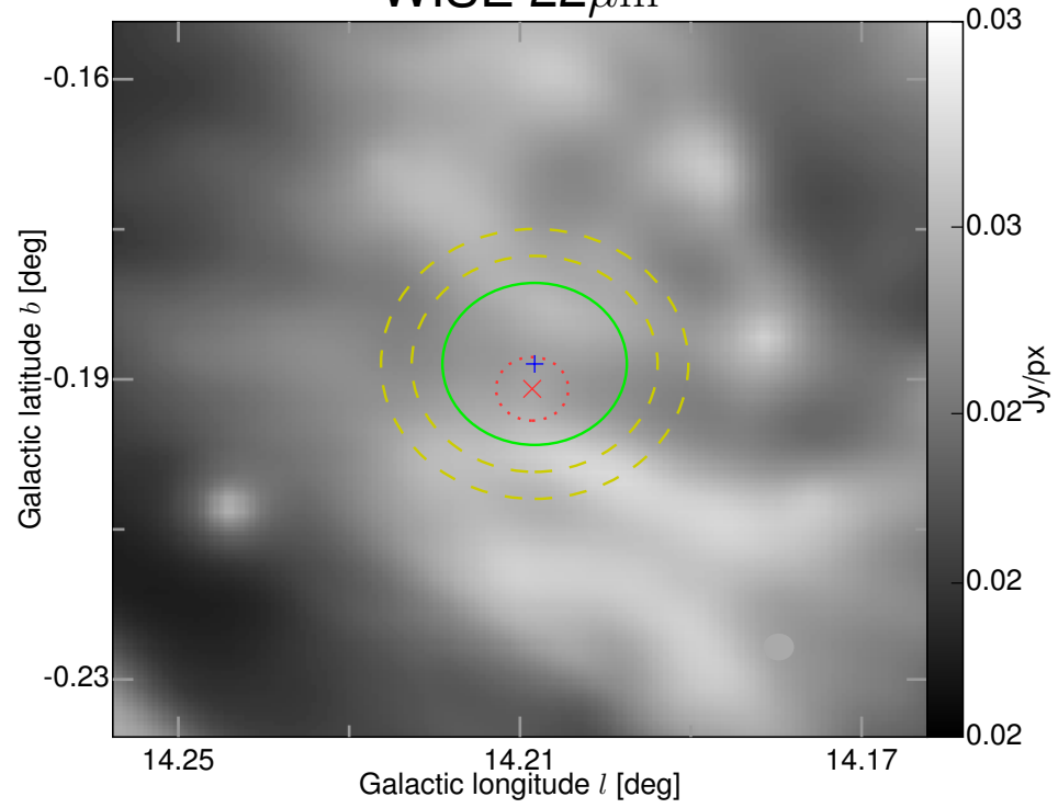
WISE 22\mu\text{m}
