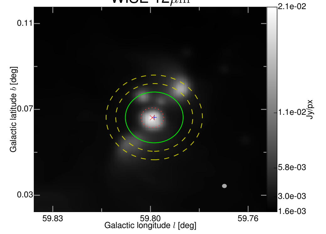
WISE 12\mu\text{m}
