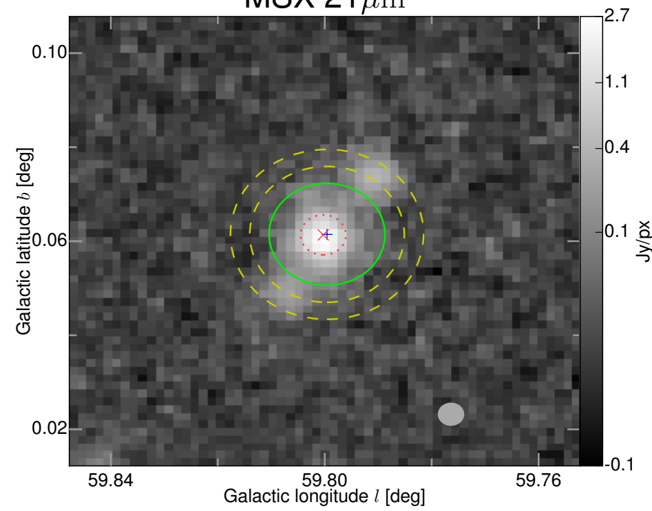
MSX 21\mu\text{m}
