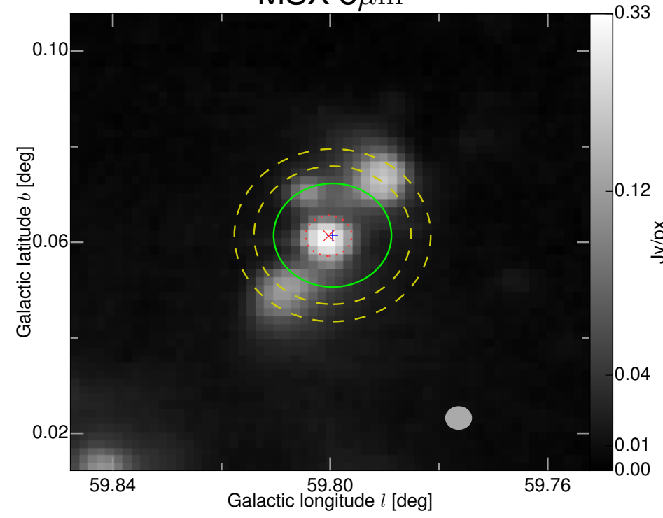
MSX 8\mu\text{m}
