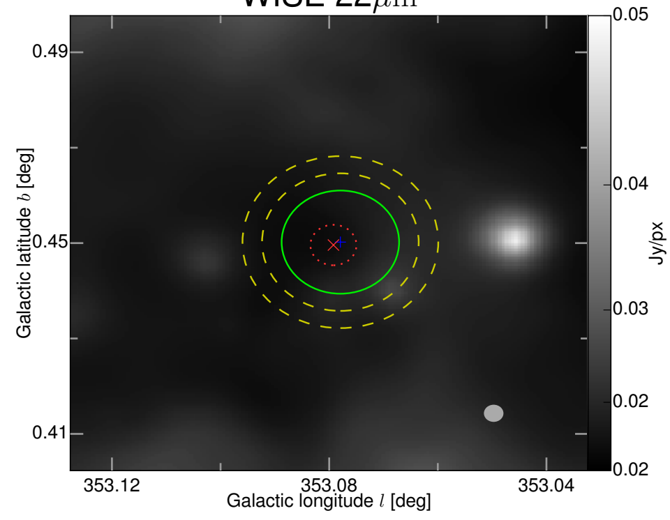
WISE 22 \mu m
