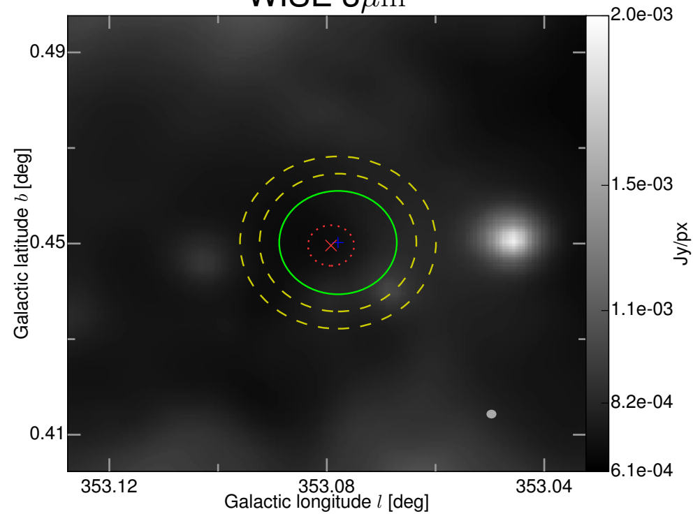
WISE 3 \mu m
