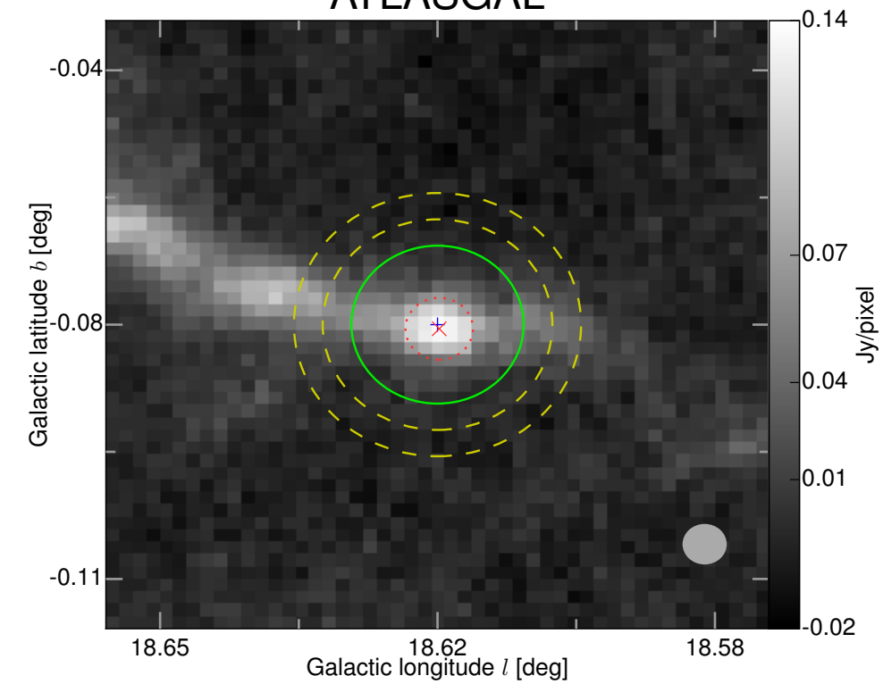
ATLASGAL
