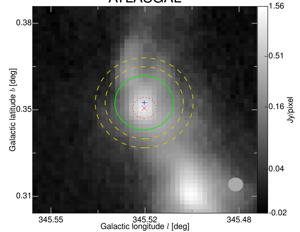
ATLASGAL
