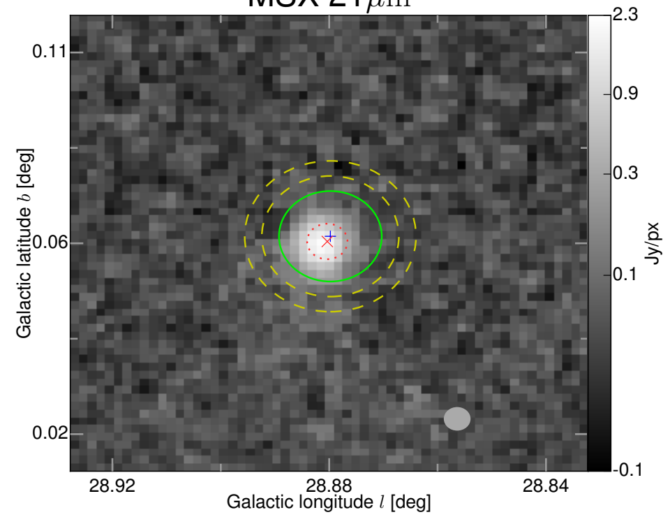
MSX 21\mu\text{m}
