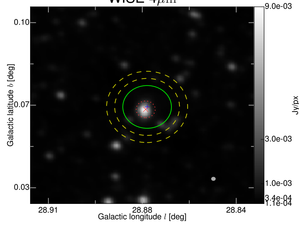
WISE 4\mu\text{m}
