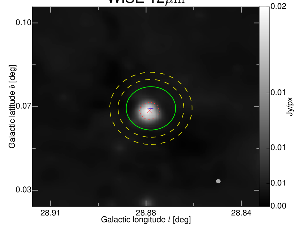
WISE 12\mu\text{m}
