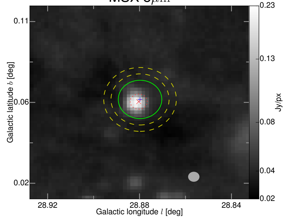
MSX 8\mu\text{m}
