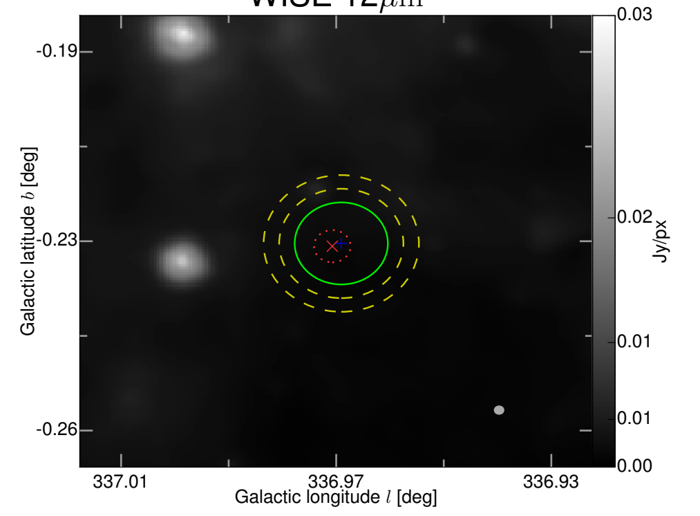
WISE 12 \mu\text{m}
