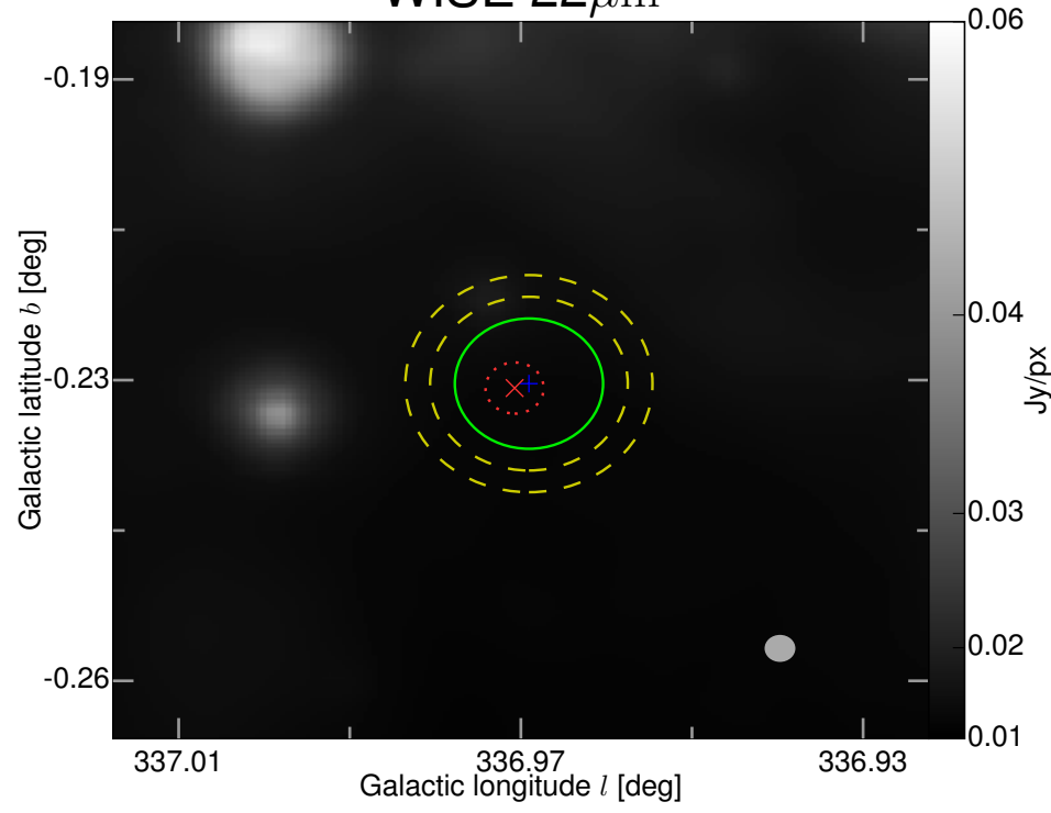
WISE 22 \mu\text{m}
