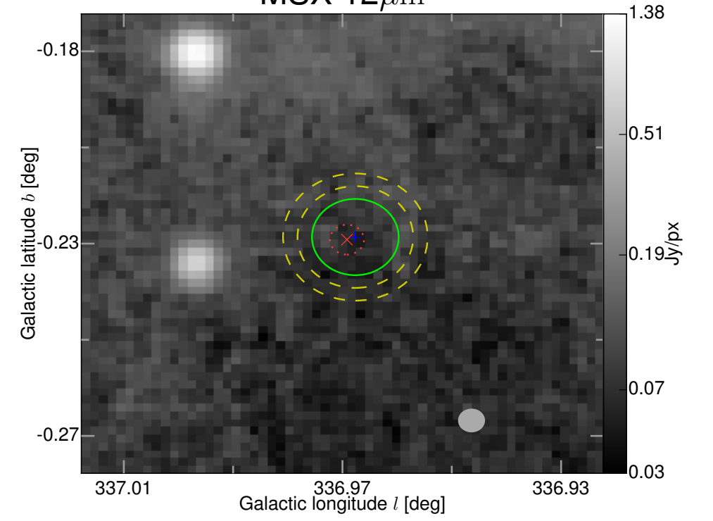
MSX 12 \mu\text{m}
