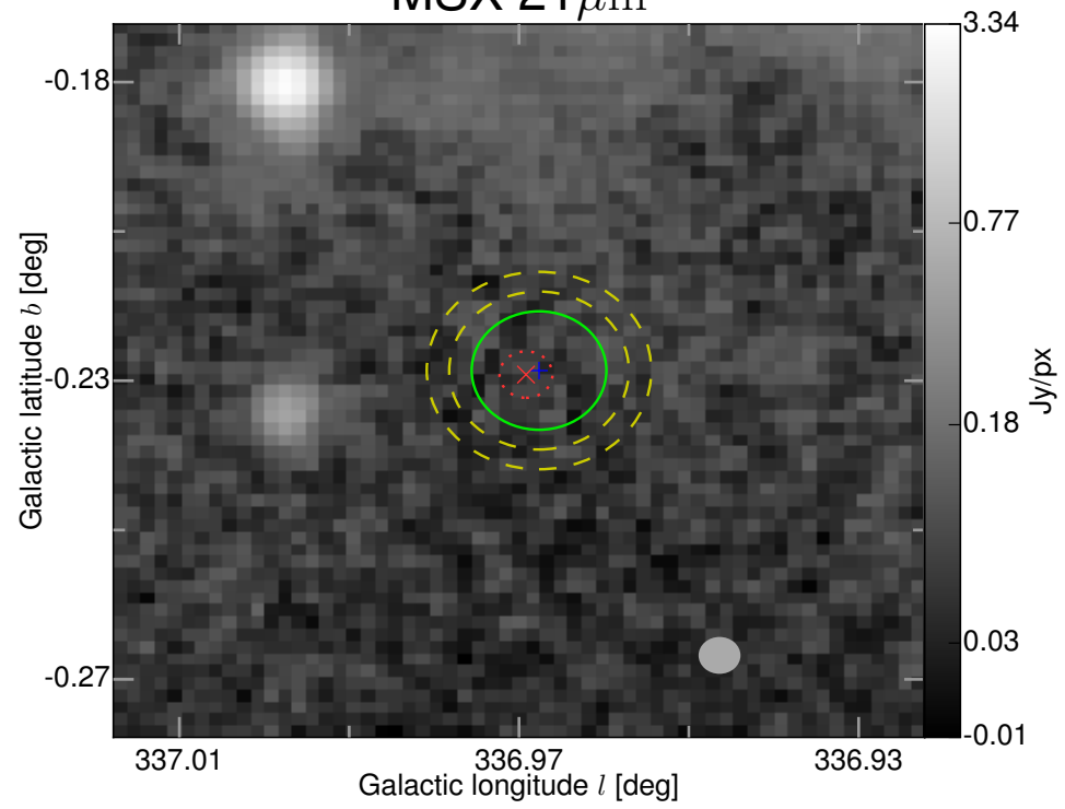
MSX 21 \mu\text{m}
